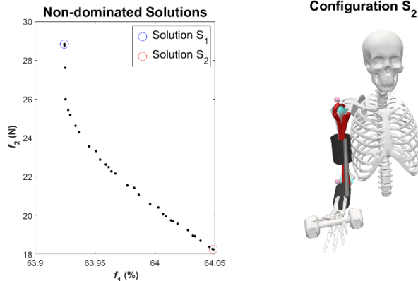
Figure 1. Multiobjective optimisation results. a) Pareto front b) S_2 actuator configuration
