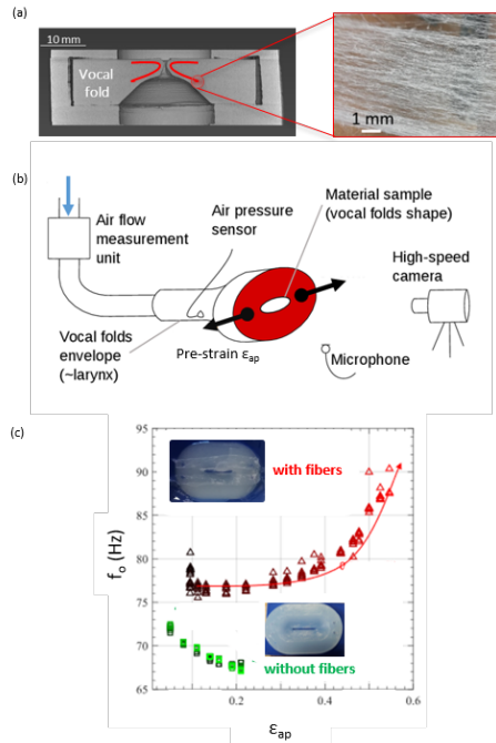
Figure 1. (a) Vocal-fold replica: mid-coronal X-ray tomographic view, scheme and zoom of an embedded PCL fibrous mat; (b) Overall in vitro testbed of phonation; (c) Fundamental frequency of oscillation against the applied anterior-posterior pre-strain.
