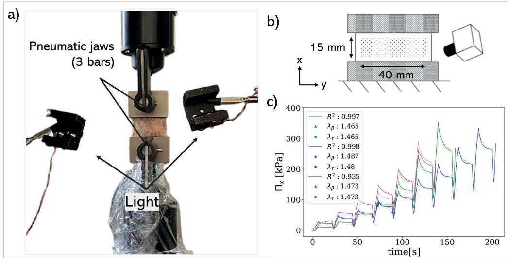
Figure 1. Device, sample geometry and pure shear stress (first Piola Kirchhoff) versus time.
