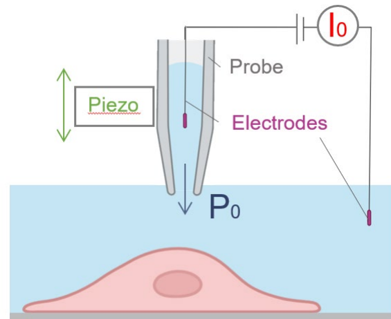
Figure 1. Schematic of the experimental SICM setup.
