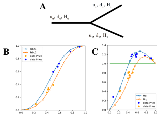
Figure 1. (A) Scheme of a junction. (B) Fractional RBC flux in function of the fractional flux at a junction. (C) Relative hematocrit in function of the fractional flux for branch 1 (blue) and branch 2 (orange). Data from Pries (1996) are superimposed. Credit: J.-M. Fullana
