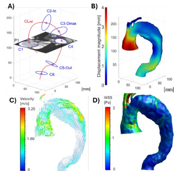
Figure 1. Illustration of results for patient 1: A) Aortic reconstruction from CLref, and 6 2D cine MRI segmented contours. B) Displacement of the aorta at the maximum volume. C) Example of a velocity vector field. D) Example of WSS map
