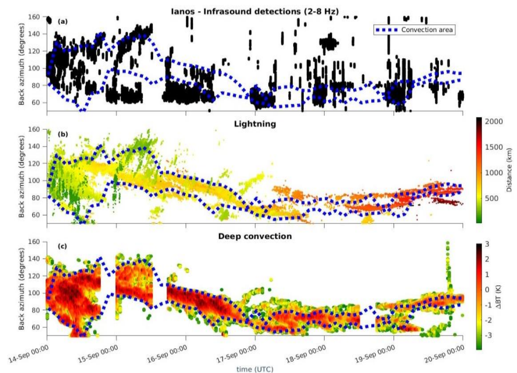
Figure 14. Same as Figure 13, but for Ianos.
