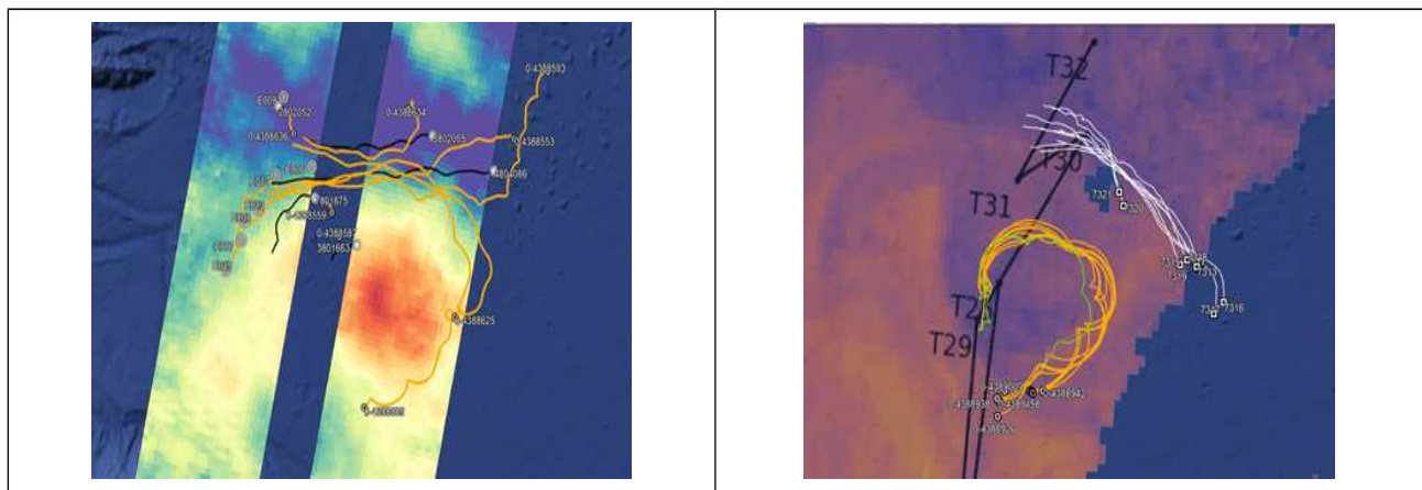
Figure 26. Left: Map of trajectories on April 29: CARTHE (orange), SVP (black), EoDyn deployment location (target symbol). The background is the SSH map from SWOT passage on 24 April. Right: Map of trajectories on 10 May: CARTHE (orange), BGC-SVP (green), CODE (white). The background is the SST map 5 May with some waypoints and ship track (black).
