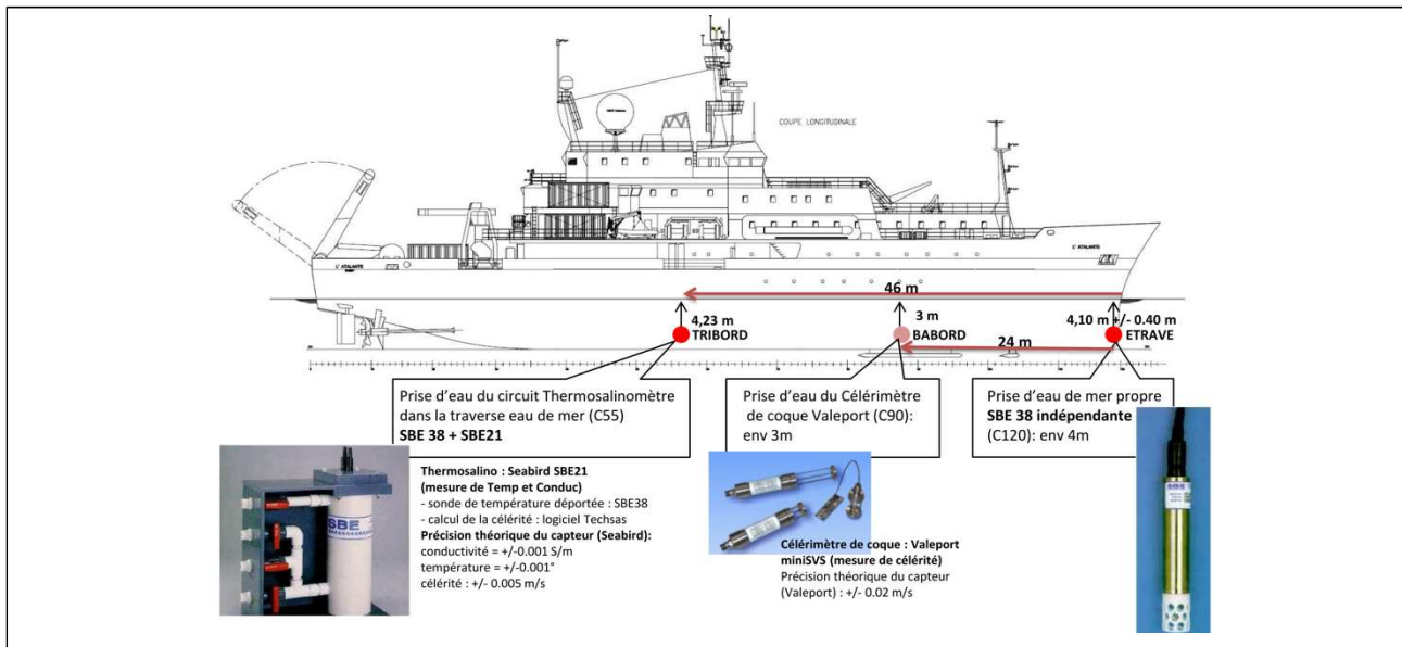
Figure 21. Positioning of the sea water intakes.
