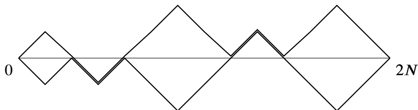
FIGURE 1. Example of a pair of reflected interfaces: k = 3 and k = 9 are contact points . At contact points, a reflection term prevents the jumps that would break the ordering to occur.
