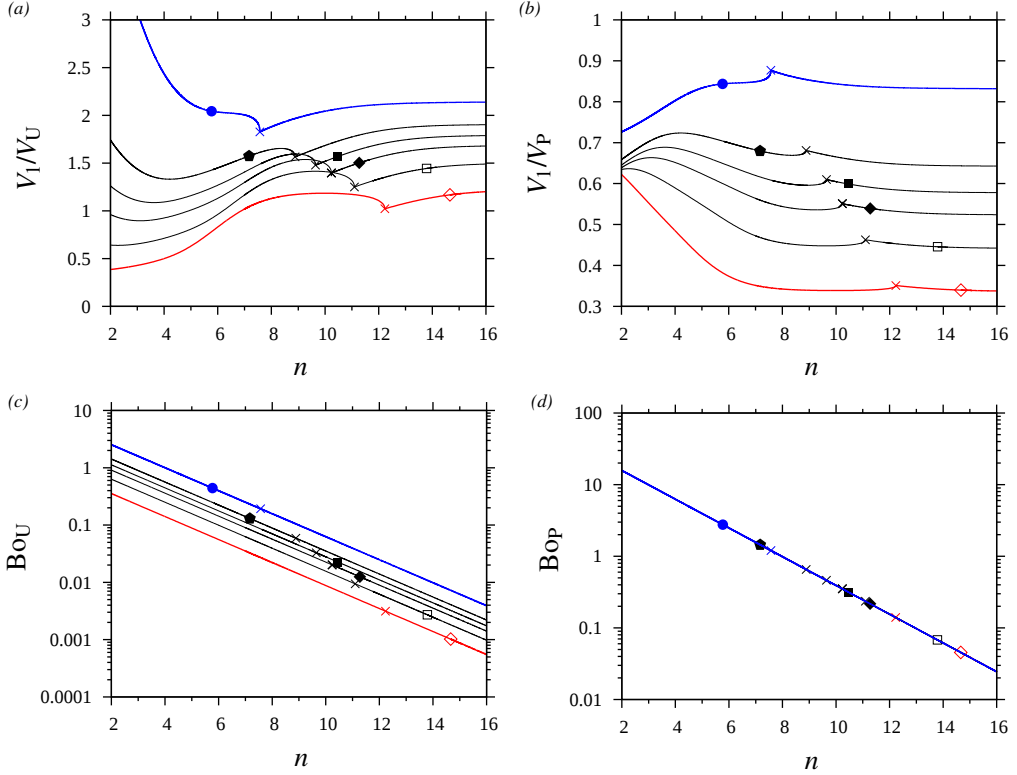
Figure 13: Liquid volume, V_1 , of TSS in figure 10a compared to different static dewetting thresholds, V_U (5.4) and V_P (5.5). From filled circles to open diamonds: h_{VE}=0.4, 0.3, 0.267, 0.24, 0.2, \text{ and } 0.15 . (a) Compared to critical volume for the existence of unduloids: V_U=1.73\pi R^3 (5.4); (b) compared to critical volume for the existence of fully-wetting spherical liquid plugs: V_P=\pi R^3(\Lambda-4/3) (5.5); (c,d) Bond numbers for liquid unduloids, Bo_U=\rho_1 g h_{VE}^{*2}/\sigma , and liquid plugs, Bo_P=Bo=\rho_1 g R^{*2}/\sigma .
