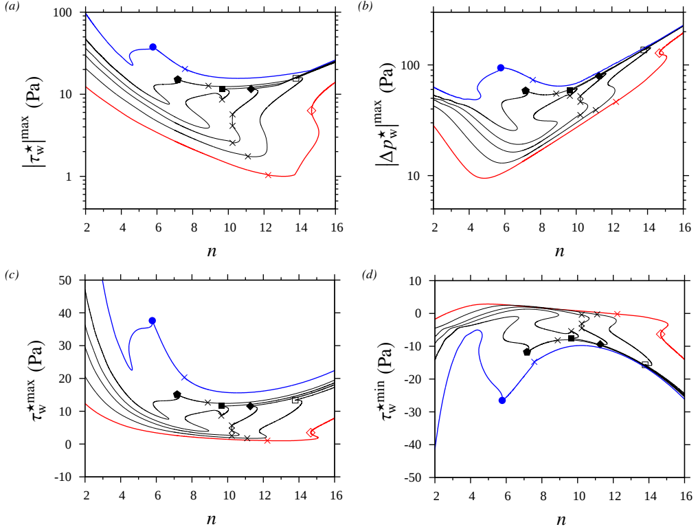
Figure 17: Wall stresses for TSS in figure 10a. Co-current configuration: Re_{20}=590 , Ka=30.6 , k=k_{\max} , R^*=R_{\text{Weib}}^* , Re_2=Re_2^{\text{Weib}} . Crosses mark CI/AI transition and other symbols correspond to LPs in figure 10a, marking the onset of TPS (except for open diamonds). Filled circles to asterisks: h_{VE}=0.4, 0.3, 0.267, 0.24, 0.2 , and 0.15 . (a) Maximum magnitude of wall shear stress, \tau_w (4.2b); (b) maximum magnitude of excess pressure, \Delta p_w (4.1); (c,d) maximum and minimum values of \tau_w .
