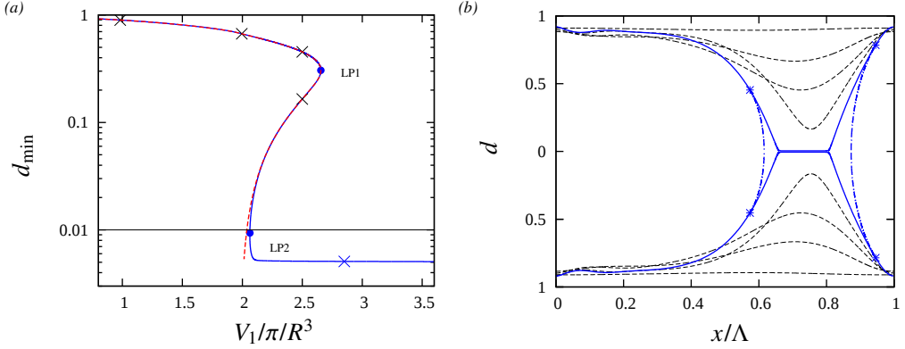
Figure 3: Transition from TWS to TPS. TSS based on our augmented WRIBL model (2.13a). Annular liquid film in contact with air within a vertical cylindrical tube: Ka=121.4 (silicone oil II and air I in table 1), R^*=1.5 mm, M=1 , \Lambda=5.4 . (a) Minimal core radius, d_{\min} , in terms of the normalized liquid volume. Solid blue: \Pi_{\text{CRL}}=\lambda=1 , d_{\text{plug}}=0.01 ; dashed red: \Pi_{\text{CRL}}=0 ; (b) profiles of TSS corresponding to crosses in panel a. Toward the tube axis: V_1/\pi/R^3=1, 2, 2.5, 2.5, 2.85 . Dot-dashed blue lines correspond to spherical-cap reconstruction (2.14) between the patching points (blue asterisks), where |\partial_x d|=\epsilon^{\max}=0.75 .
