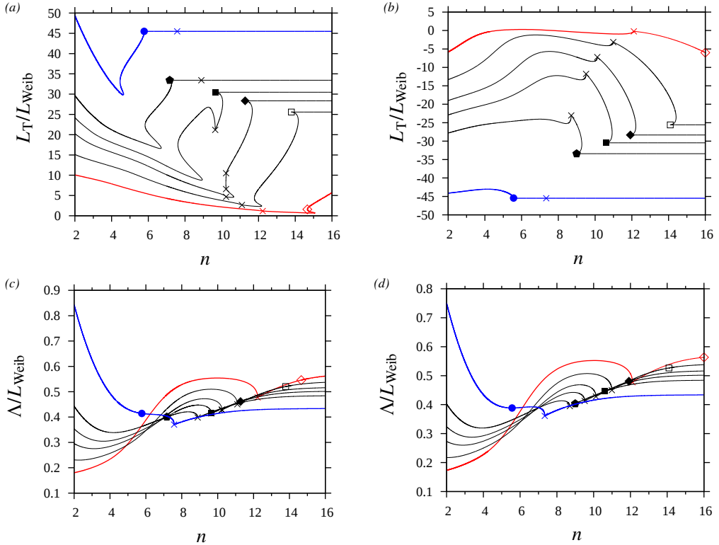
Figure 12: Length scales of TSS from figure 10, as compared to the airway length, L_{\text{Weib}} (5.1). (a,b) Relative distance of propagation, L_T/L_{\text{Weib}} , during half of one breathing period, 1/f_T , where L_T=c/2/f_T ; (c,d) relative wavelength, \Lambda/L_{\text{Weib}} . (a,c) Co-current: \text{Re}_{20}=590 ; (b,d) counter-current: \text{Re}_{20}=-590 .
