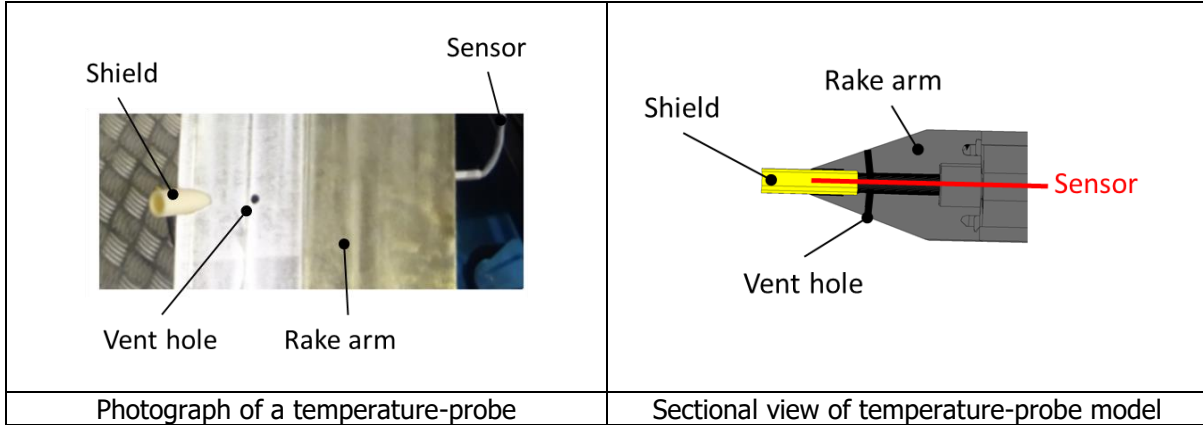
Fig 8 : Stagnation temperature-probe
