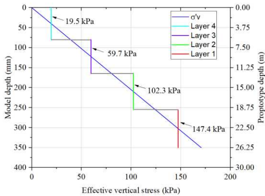
Figure 1. Applied stress for clay consolidation.
