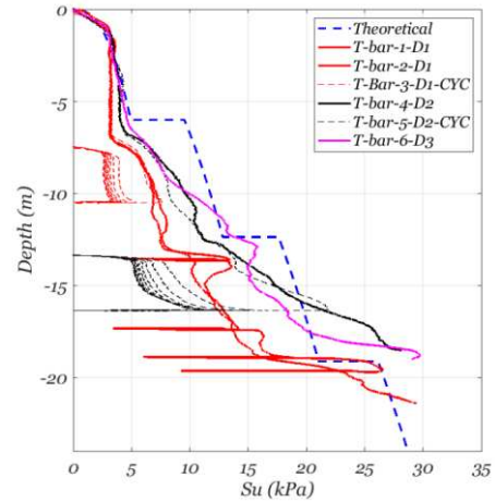
Figure 11. Profiles of undrained shear strength.
