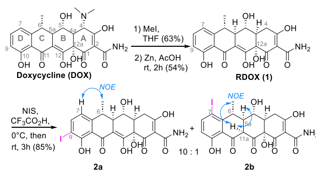
Scheme 1. Synthesis of 4- des-N -dimethyl-aminodoxycycline RDOX ( 1 ) and 9-iodo derivative 2a . Key NOE-2D NMR correlations (in blue) are shown for structural assignment of 2a and 2b .
