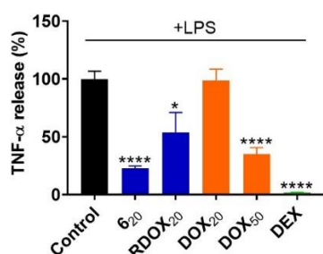
Figure 5. Anti-inflammatory effect of anti-aggregant and non-toxic tetracyclines compounds. TNF- \alpha release in primary microglial cell cultures pre-treated for 4 h with DOX, 6 , or RDOX at 20 \mu M, DOX at 50 \mu M or dexamethasone (DEX) at 2.5 \mu M, and then stimulated with 10 ng/ml of LPS for 24 h. The bars represent the mean \pm S.E.M (n = 3). Statistical analysis was performed using One-way ANOVA followed by Dunnett's test. Significant differences are indicated in the figure: * p < 0.05, **** p < 0.0001 compared to the LPS.
