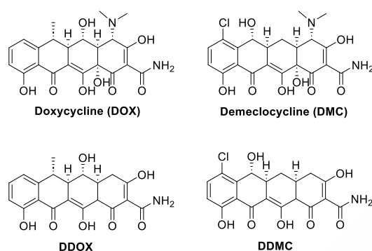
Figure 1. Structures of the reduced tetracyclines DDMC and DDOX and their respective parent compounds DMC and DOX.
