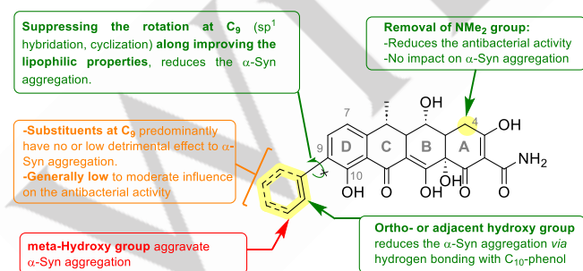
Figure 3. Summary of the SAR study concerning chemical modifications at C 4 and C 9 positions of doxycycline toward the antimicrobial and anti-aggregant properties of newly designed derivatives.
