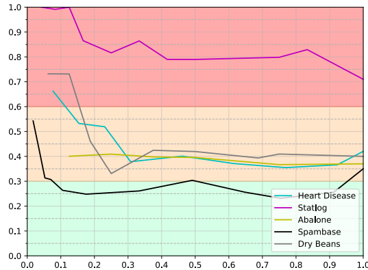
Fig. 10: \max(q^{acc}, q^{f1}) as a function of \frac{\#Features}{\#MaxFeatures} when we reduce Data Dimensionality by removing features.
