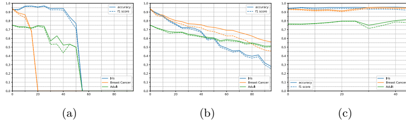
Fig. 2: Evolution of mean accuracies and f1-scores when errors are injected in Iris, Cancer, and Adult: missing values (a), outliers (b), and fuzzing (c).
