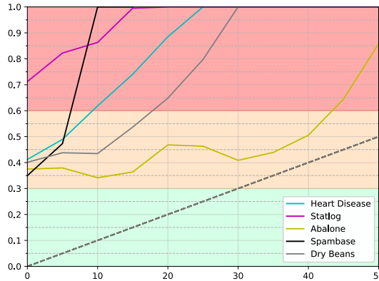
Fig. 8: \max(q^{acc}, q^{f1}) when missing errors are injected in data (solid lines) and the completeness ratio (dashed lines).
