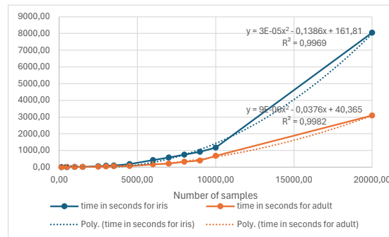
Fig. 11: Variation of the computational time (in seconds) as a function of dataset sizes
