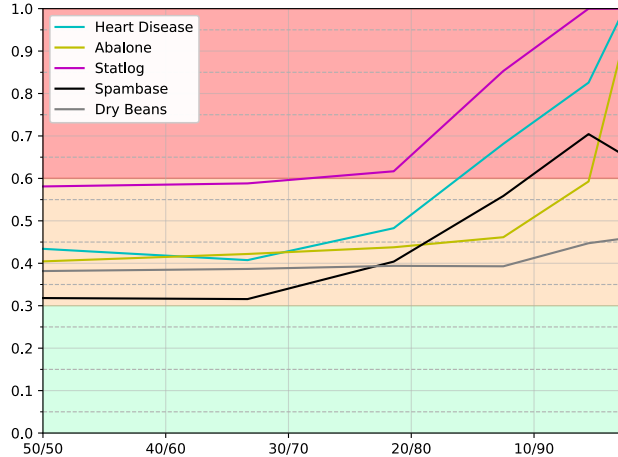
Fig. 9: \max(q^{acc}, q^{f1}) on datasets having an imbalance ratio given by the x-axis.
