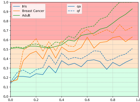
Fig. 4: Evolution of q^{acc} (solid lines) and q^{f1} (dashed lines) with imbalanced classes for Iris, Breast Cancer, and Adult. The horizontal axis shows the percentage of samples removed in one class
