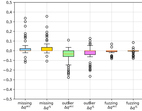
Fig. 7: Summary of the distributions of \Delta q_{e,p}^{acc}(D) and \Delta q_{e,p}^{f1}(D) for 0% to 50% of missing values, outliers and fuzzing.
