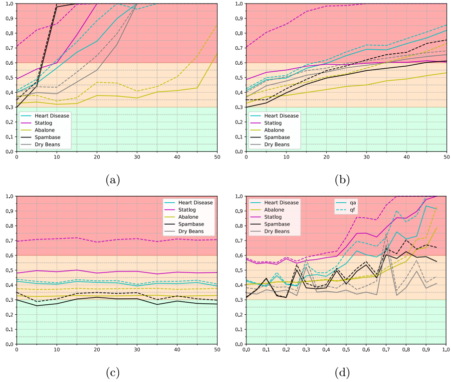
Fig. 5: q^{acc} (solid curves) and q^{f1} (dashed curves). The x -axis shows datasets with x percents of deterioration for a) missing values, b) outliers, c) fuzzing and d) class imbalance.
