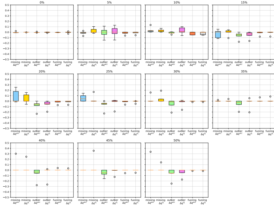
Fig. 6: Distributions of \Delta q_{e,p}^a(D) and \Delta q_{e,p}^{f1}(D) detailed for every 5% increment of missing values, outliers and fuzzing up until 50%.
