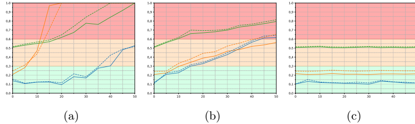
Fig. 3: Evolution of q^{acc} (solid lines) and q^{f1} (dashed lines) when errors are injected in training data (missing values (a), outliers (b), and fuzzing (c)).
