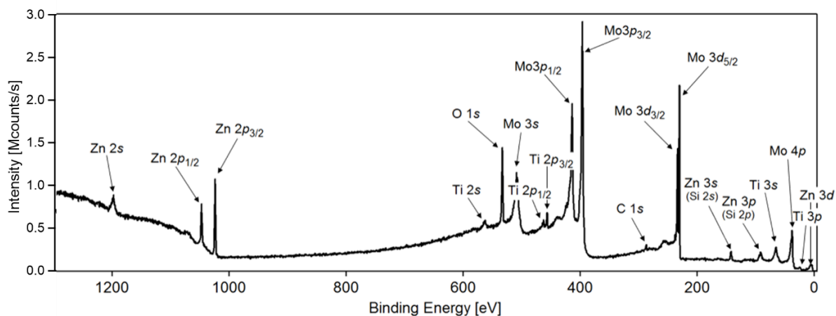
Fig. 3. HAXPES wide scan of as deposited 29.7@RT sample. Only core level peaks are visible since Auger lines are found at higher binding energies.
