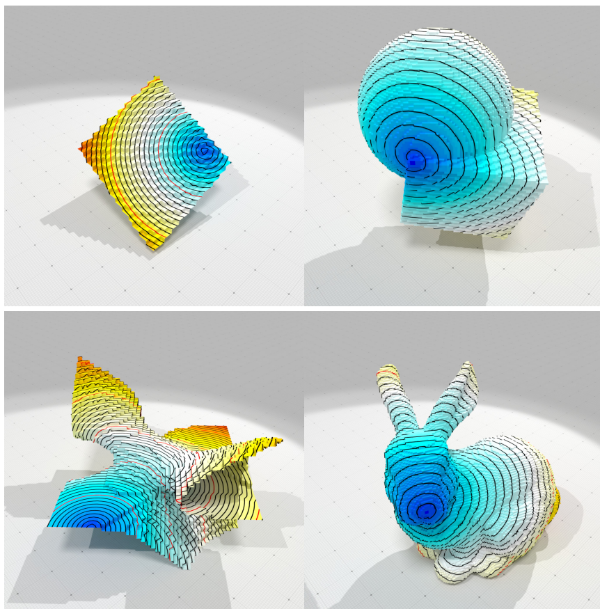
Fig. 7 Illustration of geodesics onto digital sets (source in deep blue).
