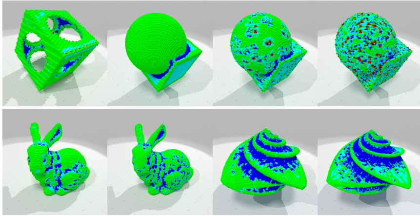
Fig. 4 Raw multiscale local shape geometry analysis (green: convex, blue: concave, red: atypical, cyan: planar), with a maximal scale of 5.
