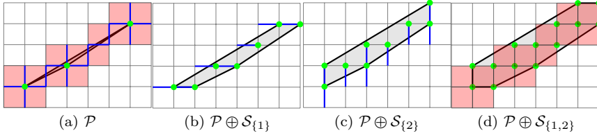
Fig. 2 Let \mathcal{P} = \text{cvxh}(\{(0, 0), (2, 1), (5, 3)\}) . (a) \mathcal{C}^d[\mathcal{P}] . (bcd) We can see that \#(\mathcal{C}_{\{1\}}^d[\mathcal{P}]) = \#(\mathcal{C}_0^d[\mathcal{P} \oplus \mathcal{S}_{\{1\}}]) = 7 , \#(\mathcal{C}_{\{2\}}^d[\mathcal{P}]) = \#(\mathcal{C}_0^d[\mathcal{P} \oplus \mathcal{S}_{\{2\}}]) = 9 , and \#(\mathcal{C}_{\{1,2\}}^d[\mathcal{P}]) = \#(\mathcal{C}_0^d[\mathcal{P} \oplus \mathcal{S}_{\{1,2\}}]) = 14 . The bijections \mathcal{Z}_{\{1\}} , \mathcal{Z}_{\{2\}} , \mathcal{Z}_{\{1,2\}} are made clear in (b), (c), (d) respectively.
