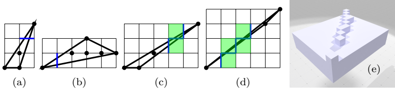
Fig. 1 (abcd) Digital triangles that are not fully convex: digital points are depicted as black disks, missing 1-cells for digital 1-convexity as blue lines, missing 2-cells for digital 2-convexity as green squares. (e) Usual digital convexity (1) plus 3D connectivity does not imply connectedness on the upper slice; it is also not fully convex.
