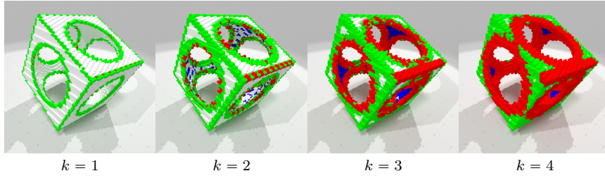
Fig. 3 Local shape geometry analysis at fixed scale (green: k -convex, blue: k -concave, red: k -atypical, white: k -planar). One easily see that k -atypical implies (k + 1) -atypical, while k -convex implies (k - 1) -convex and k -concave implies (k - 1) -concave.
