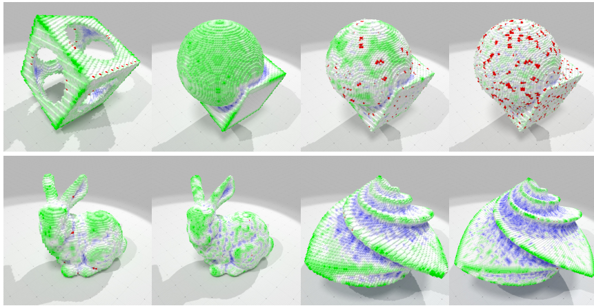
Fig. 5 Smooth multiscale local shape geometry analysis (green: convex, blue: concave, red: atypical, white: planar), with a maximal scale of 5. For a convex zone, the saturation of green is the ratio (a_X(z) - b_X(z))/5 . For a concave zone, the saturation of blue is the ratio (b_X(z) - a_X(z))/5 .
