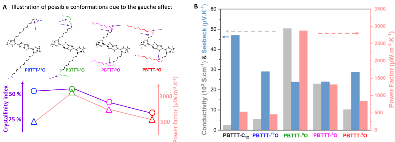
Fig. 3 A. Illustration of possible conformations related to the gauche effect, showing the evolution of the disorder associated with the position of the oxygen along the side chain. The arrows indicate the gauche effects represented on each side chain. Evolution of crystallinity index and power factors are illustrated as function of the position of the oxygen along the side chain B. TE properties of doped polymer thin-films ( [\text{F}_6\text{TCNNQ}] = 5 \text{ mg}\cdot\text{mL}^{-1} ) measured in parallel to the rubbing direction (color code: electrical conductivity, Seebeck coefficient and power factor).
