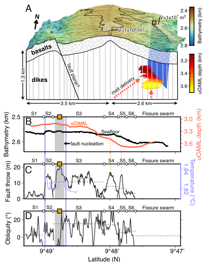
Fig. 5. Tectono-magmatic link of the oblique-trending F_3 at 9^\circ 48' N . (A) Three-dimensional ridge-perpendicular schematic diagram showing the main features of the seafloor and the subseafloor and lava flow outline, based on AUV high-resolution bathymetry and seismic volume. The orange square marks the location of the fault nucleation. The potential fault plane obtained as an extension of its surface expression in depth (not imaged in seismic) is shown on the west flank in dashed line. The lava volume emplaced on the seafloor through this fault system (white shaded area) is estimated as 1 \times 10^7 \text{ m}^3 , using the “PILE VOLUME” of Global Mapper software. The lava volume near the AST (white shaded area) was estimated as 1 \times 10^6 \text{ m}^3 (23). Dashed red arrows indicate potential melt delivery pathways from the main AML (arrow on the left of the uOAML) and from previously reported lower crustal OAMLs (44). (B) Depths of the seafloor and uOAML along the F_3 . The gray shaded zone marks the fault nucleation zone. (C and D) Fault throw and obliquity along the F_3 , respectively. The pale purple line in panel (C) shows measured temperature along the northernmost part of the fault scarp recorded on the probe closest to the seafloor (SI Appendix). The two vertical bars in the same color delimit the latitudinal extent of the higher temperature anomaly. Vertical dashed orange lines mark correlation between higher fault throws and abrupt changes in the uOAML depth for segments S4 and S5. Gray dashed lines show the average values for each fault segment (S1–S6). The average obliquity of the fissure swarm is also included.
