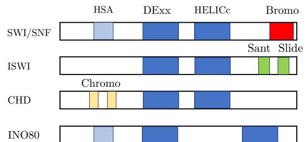
FIG. 1. Schematics of the four remodeler families as defined by domain composition. All remodelers contain two ATPase domains (DExx, HELICc), shown in dark blue, and accessory domains of regulatory purposes: the bromodomain (red), chromodomain (yellow), sant-slide domains (green) and the actin-binding domain HSA (light blue). Redrawn after (Clapier and Cairns 2009).
