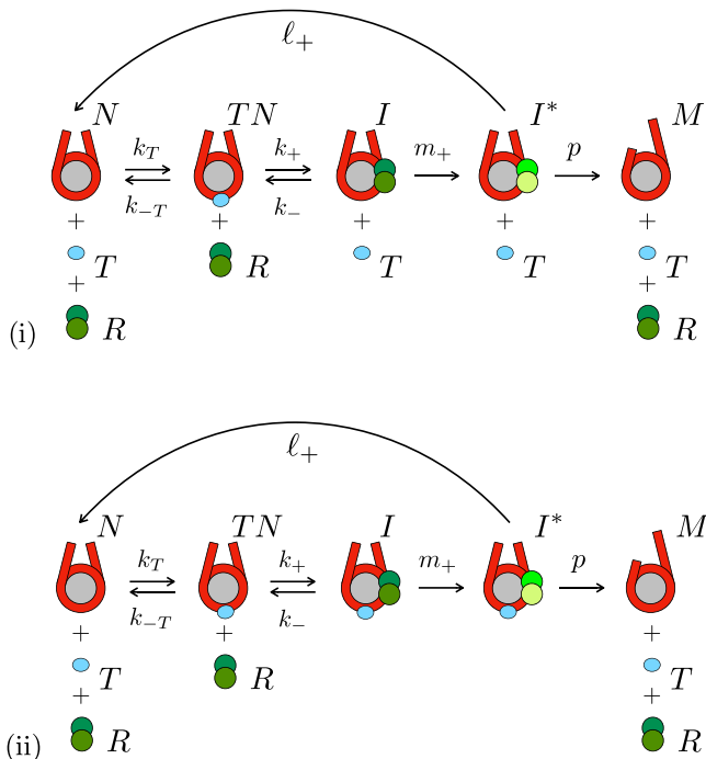
FIG. 3. Kinetic proofreading scenarios (i) and (ii) of chromatin remodeling in its latest version. N denotes the nucleosome, T is a pioneer transcription factor, R is the remodeler; I and I^* are remodeler-nucleosome complexes; M is the mobile nucleosome. For the interpretation, see main text. Reprinted with permission from the American Physical Society (Schiessel and Blossey 2020).
