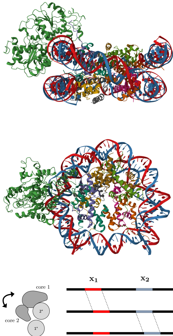
FIG. 2. Cryo-EM structure of the ISWI-ATPase-nucleosome complex discussed in (Chittori et al. 2019). Taken from the PDB, entry 6PFW. The top image shows the side view, in which the two domains, or cores, are clearly discernable. The middle image shows the top view of the nucleosome-remodeler complex. The bottom image illustrates the mapping of the remodeler action on the nucleosome to the molecular motor model of a Brownian dimer. \mathbf{x}_1 (red) and \mathbf{x}_2 (blue) are the footprints of the remodeler cores on the DNA. This figure is redrawn after (Blossey and Schiessel 2019).
