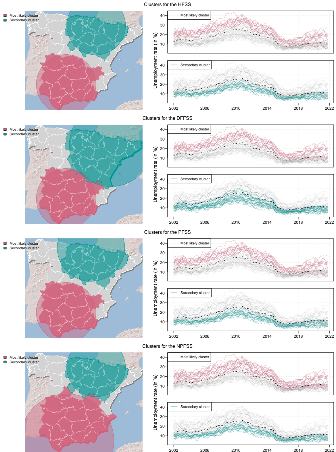
Figure 3: Clusters for the HFSS, DFSS, PFSS, NPFSS methods, for the variable Unemployment rate (in %), observed quarterly from 2002 to 2022 in Spain.
