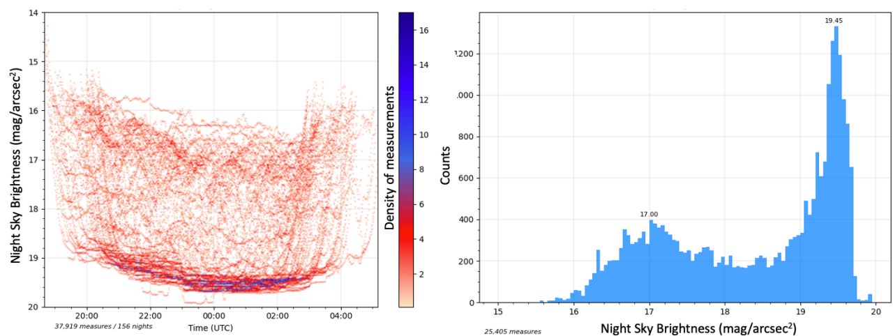
Fig. 3. NSB measured with NINOX for the OSUG site from April to September 2024. Left: Density plot combining measurements on moonless nights. Right: Histogram of the measurements from the left plot excluding twilights.
