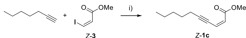
Scheme 4. Synthesis of analogs Z-1c . Reagents and conditions: i) PdCl 2 (PPh 3 ) 2 , CuI, Et 3 N, THF, 0 °C to rt, 67%.
