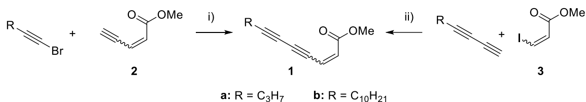
Scheme 3. Synthesis of Lachnophyllum methyl esters Z-1a and E-1a and analogs Z-1b and E-1b . Reagents and conditions: i) Cadiot-Chodkiewicz coupling: CuCl, NH 2 OH·HCl, n BuNH 2 , THF, 0 °C to rt; ii) Sonogashira coupling: PdCl 2 (PPh 3 ) 2 , CuI, Et 3 N, THF, 40 °C overnight.
