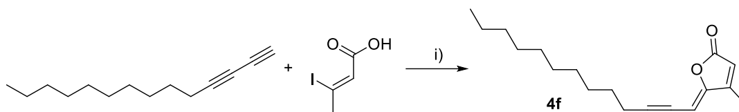
Scheme 9. Synthesis of (4Z)- Lachnophyllum lactone analog 4f . Reagents and conditions: i) \text{PdCl}_2(\text{PPh}_3)_2 , CuI, \text{Et}_3\text{N} , \text{CH}_3\text{CN} , 40^\circ\text{C} overnight, 35%.
