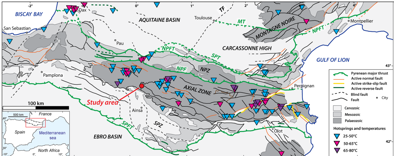
Figure 1. Structural map of the Pyrenees showing the main faults and structural domains. Current hot springs and associated temperatures are reported with coloured triangle shapes (modified after Eude et al., 2020). The study area along the Pic de Port Vieux thrust (PPVT) in the Axial Zone is indicated by a red dot.
