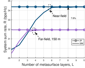
Fig. 2. The system sum rate versus L under near-field and far-field channel. ( S = K = 4 and P_T = -40 dBm).
