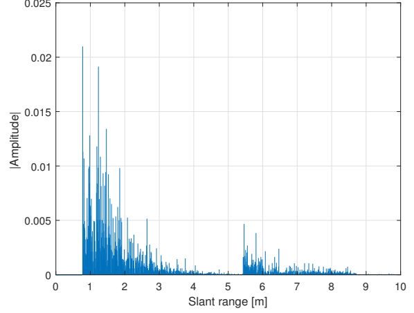
Fig. 2: Impulse response of a LOS industrial indoor environment simulated according to IEEE 802.15.4a CM7 model
