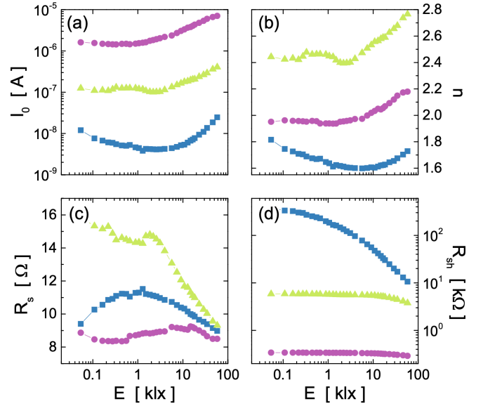
FIG. 2. (a, b, c, d) Fitting parameters of the single-diode electrical model, I_0 , n , R_s and R_{sh} respectively vs illuminance. The data of three CIGS cells are plotted with the following compositions: GGI = 0.28 , CGI = 0.94 (purple dots), GGI = 0.81 , CGI = 0.99 (green triangles) and GGI = 0.28 , CGI = 0.47 (blue squares).
