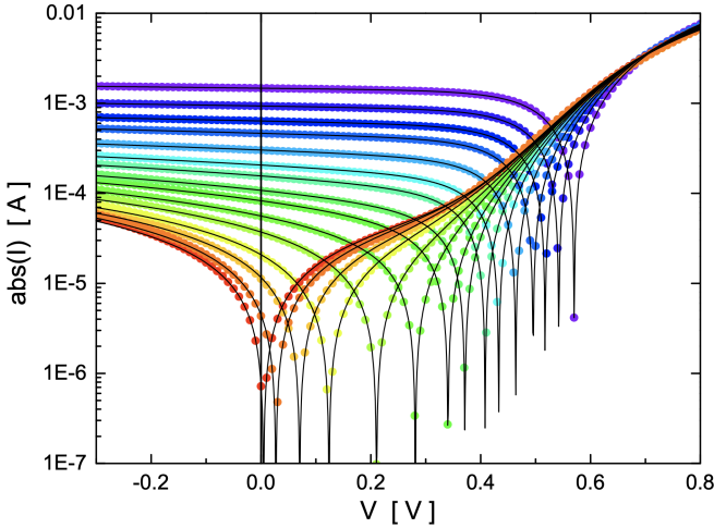
FIG. 1. Current-voltage characteristics measured in a CIGS cell with GGI = 0.81 and CGI = 0.99 as a function of the illuminance of a white LED in the range 50 lx to 60 klx. The dots are the experimental data and the solid lines are the fits by the single-diode model.
