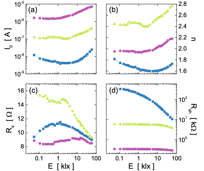
FIG. 2. (a, b, c, d) Fitting parameters of the single-diode electrical model, I_0 , n , R_s and R_{sh} respectively vs illuminance. The data of three CIGS cells are plotted with the following compositions: GGI = 0.28 , CGI = 0.94 (purple dots), GGI = 0.81 , CGI = 0.99 (green triangles) and GGI = 0.28 , CGI = 0.47 (blue squares).
