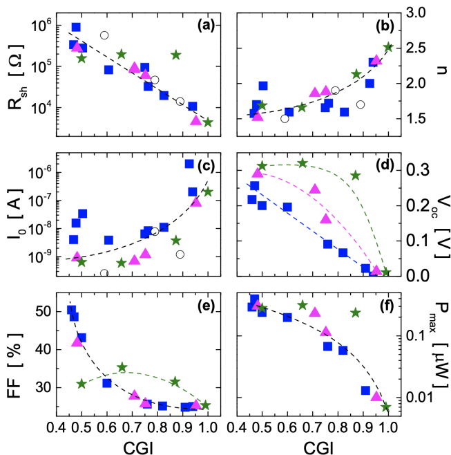
FIG. 5. Fitting parameters from the illuminance dependence of the IV curves vs the CGI ratio for the three cell series with GGI ratios equal to 0.28, 0.64 and 0.81 (square, triangle and star symbols respectively) : (a) R_{sh} , (b) n and (c) I_0 . The open circles are from Ref. 5 . The open circuit voltage (d), fill factor (e) and maximum power (f) measured for an illuminance of 100 lx. Dashed lines are guides for the eyes.
