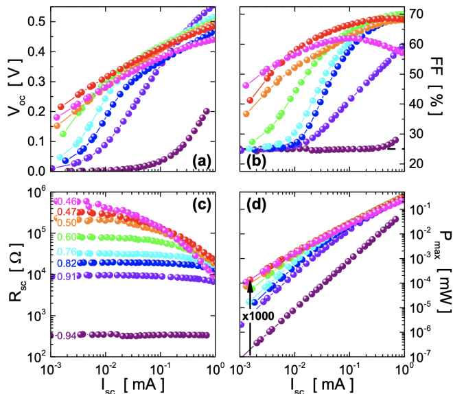
FIG. 3. (a), (b), (c) and (d) Open circuit voltage, fill factor, short circuit resistance and maximum power as a function of the short circuit current for 8 photovoltaic cells. The CIGS absorbers have an average GGI ratio of 0.28 and CGI ratios in the range 0.46 – 0.94, which are indicated in (c).
