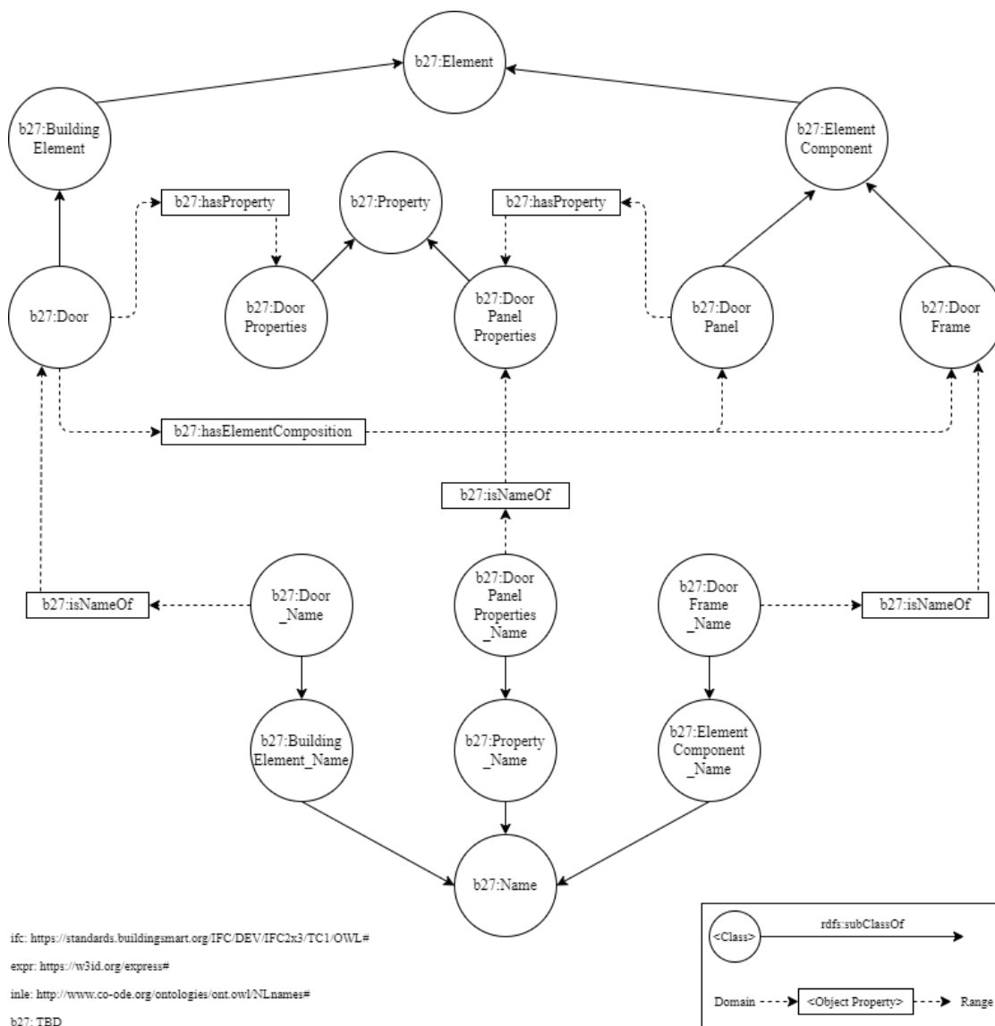
Figure 2: Simplified view of the TBox of our OB27AI ontology.
