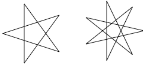
Figure 5. – A (5, 2) and (7, 3) star polygon.
