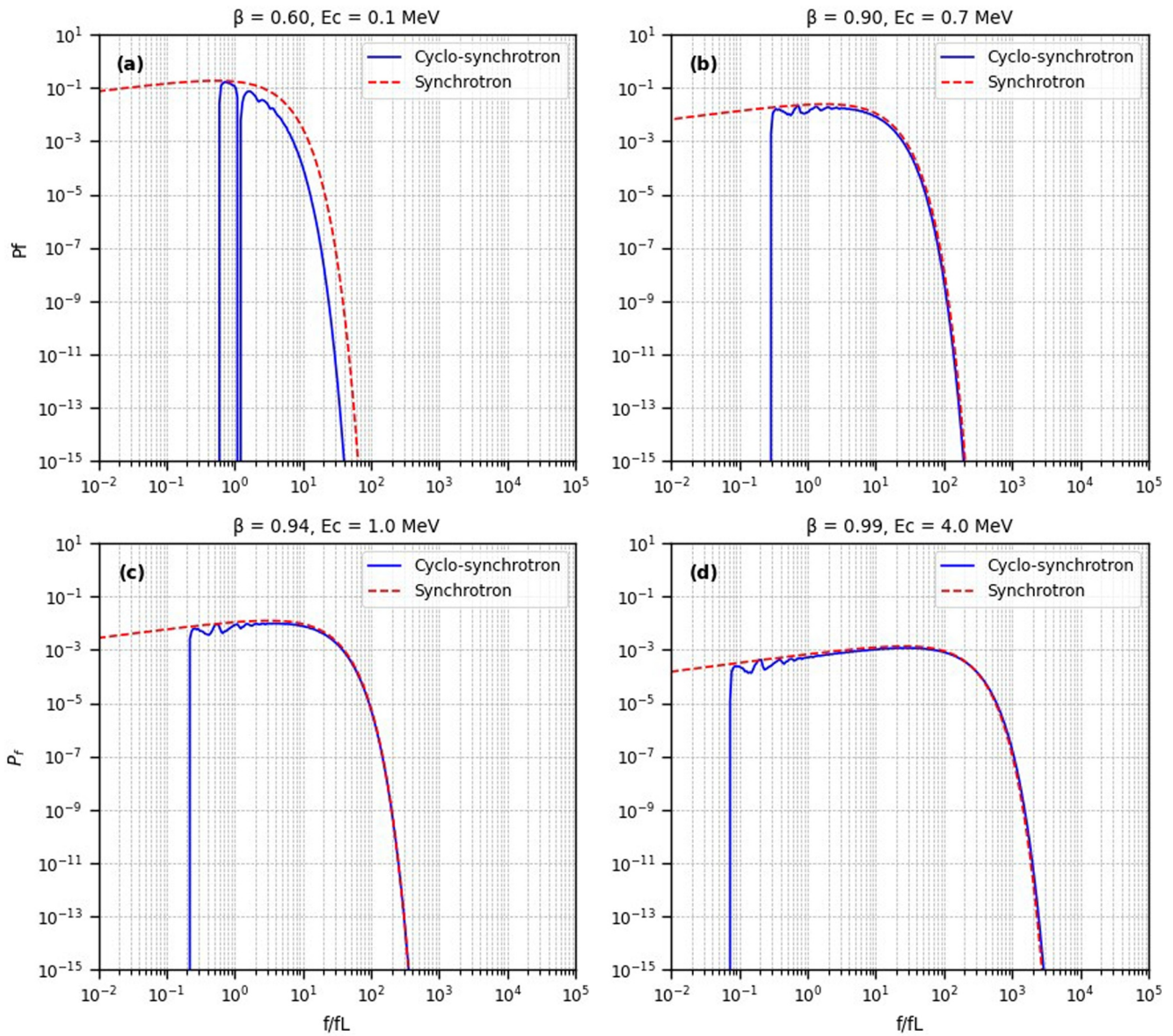
Figure 2. Plots of normalized emission as a function of f/fL for (a) \beta = 0.6 , (b) \beta = 0.9 , (c) \beta = 0.94 , (d) \beta = 0.99 and an observation angle of \theta = \pi/3 . The plain line corresponds to the cyclo-synchrotron emission of an isotropic distribution after integration over the pitch angle \alpha given in Equation 11. The dashed line corresponds to the synchrotron emission given by Equation 3.
