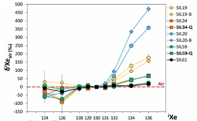
Fig. 9. Isotopic spectra of Xe from the total gas released during the experiment of each sample of Siljan (Supp. Table 1). Isotopic compositions are given using the delta notation normalized to ^{130}\text{Xe} and to the isotopic composition of the modern atmosphere (Ozima and Podosek, 2002) ( \delta^i\text{Xe}_{\text{air}} = 0 \% ):
