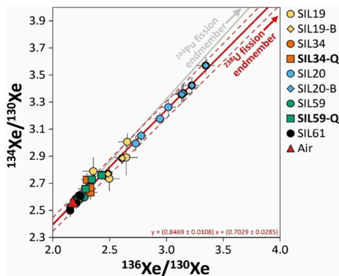
Fig. 11. Three-isotope plot of Xe for crushing experiments on Siljan samples (see data in Supp. Table 1). According to the slope of the linear regression on the results obtained on Siljan samples, data plot along the mixing line (red line) between air and the pure ^{238}\text{U} fission endmembers (Porcelli and Ballentine, 2002), not on the mixing line (grey line) between air and the pure ^{244}\text{Pu} fission endmembers. The slope defined by the data from Siljan ( 0.847 \pm 0.011 ) matches the ^{134}\text{Xe}/^{136}\text{Xe} ratio produced by the fission of the ^{238}\text{U} ( 0.832 \pm 0.012 , Ozima and Podosek, 2002; Porcelli and Ballentine, 2002). The dashed lines represent the uncertainty at 1\sigma of the mixing line. (For interpretation of the references to colour in this figure legend, the reader is referred to the web version of this article.)
