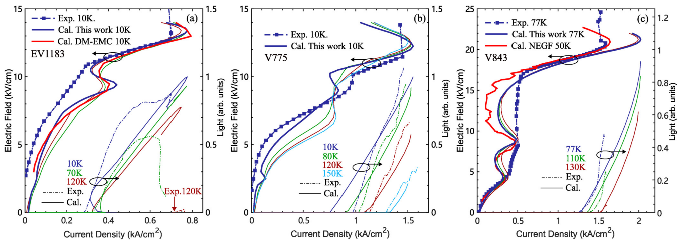
FIG. 7. L - I - V curves of the three structures from the model in this work, experiments, and other models. (a) EV1183: experiment data are extracted from Ref. 84, and DM-EMC result is from Ref. 15. (b) V775: experiment measurement is from Refs. 62 and 85. (c) V843: experiment data from Ref. 86, and NEGF calculated in Ref. 70.
