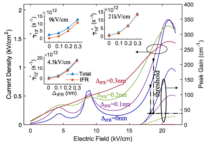
FIG. 9. I - V and peak optical gain vs the electric field of V843 for varying \Delta_{\text{IFR}} from 0 to 0.3 nm, \Delta_{\text{IFR}} = 10 nm. The three insets are the total and IFR pure dephasing rate of 1-2', 1-3', and 1-4' at their alignment electric field of 4.5, 9, and 21 kV/cm, respectively.
