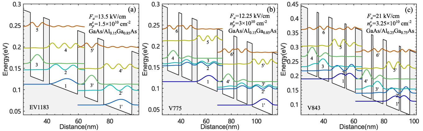
FIG. 6. Conduction band potential profile and probability densities offset by the eigenenergies of the investigated structures (two periods). Bias, sheet carrier density per period, material composition, and wafer number are reported. (a) Two-well resonant phonon device (EV1183). 84 (b) Three-well resonant phonon device (V775). 62 (c) Four-well indirect pumped phonon-photon-phonon device (V843). 70
