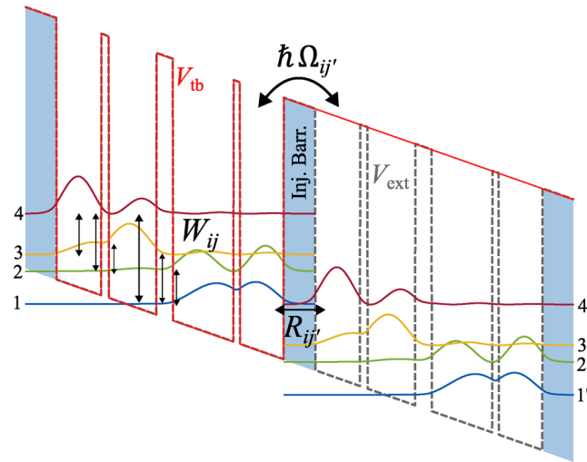
FIG. 2. Carrier transport model description. Two adjacent modules of a QCL are separated by the injection barrier (blue shaded area), with the tight-binding potential of the left period (solid red line) and extended potential (dashed grey) reported. Intra-module carrier transport is driven by inter-subband scattering. The coupling of two adjacent modules is described using coupling strength. The inter-module tunneling rate can be calculated with the detuning energy and the dephasing rate. The structure is from Ref. 70.
