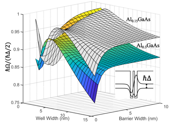
FIG. 4. The ratio between the calculated coupling strength and the exact value. The calculated value is obtained between the localized ground basis of two coupled QWs under tight-binding Hamiltonian from Eq. (13). The exact result is half of the detuning energy between the coupled states obtained by extended well-defined Hamiltonian as illustrated in the inset. The grey surface is for the Al 0.15 GaAs barrier, and the colored surface is for the Al 0.3 GaAs barrier.
