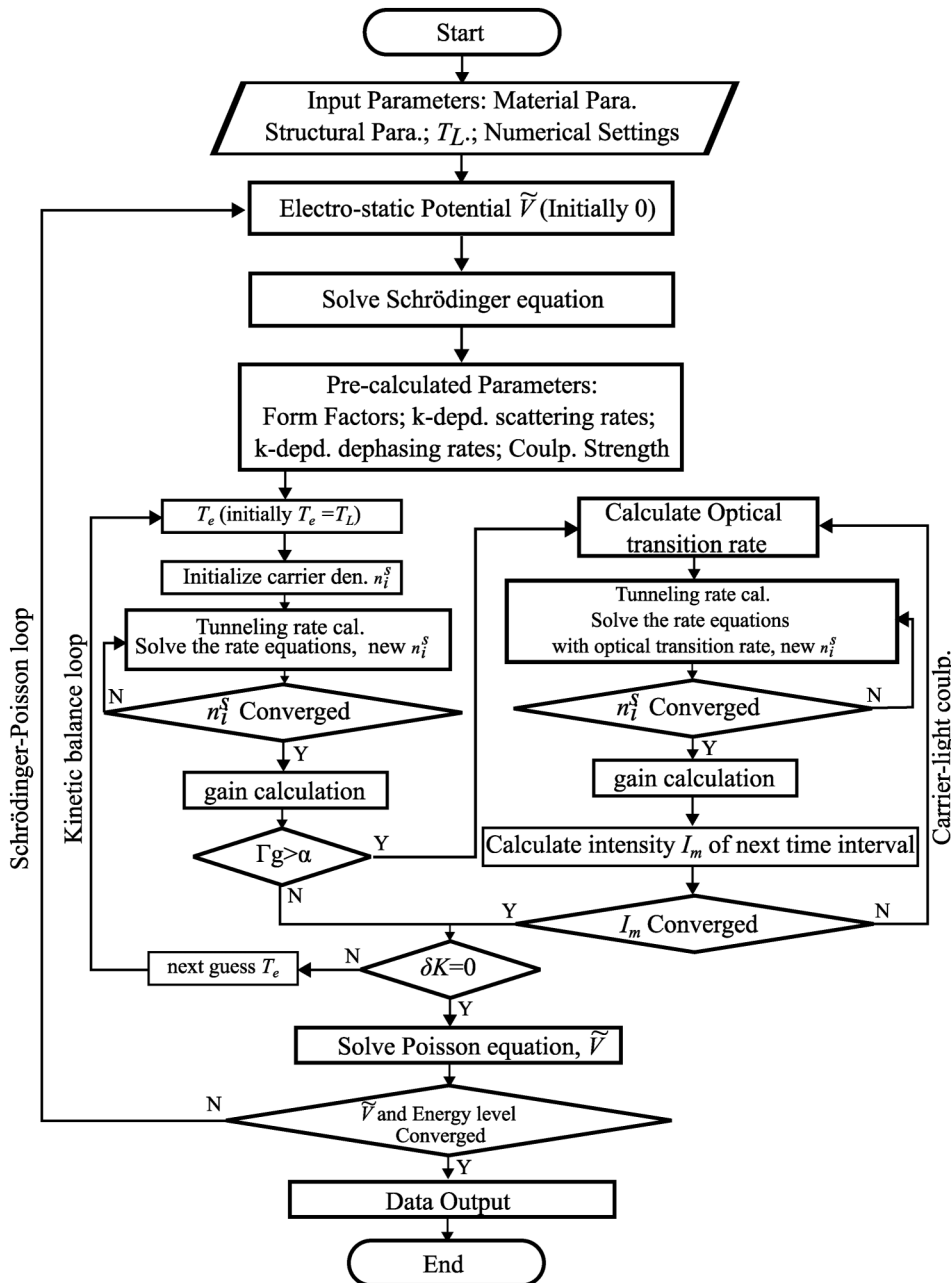
FIG. 12. Simplified flow chart of the model in this work.
