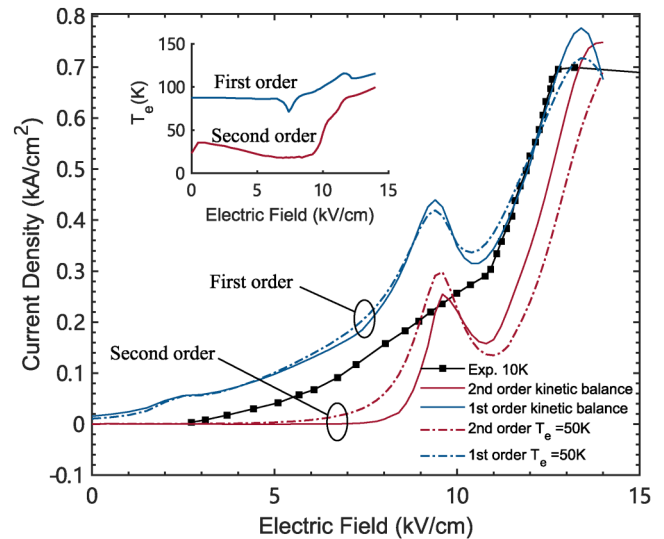
FIG. 11. I - V comparison between first-order and second-order current approximation of the device EV1183, with kinetic balance and by assuming a constant electron temperature of 50 K. The lattice temperature is set to be 10 K in this test. The inset is the electron temperature estimated by the two methods.
