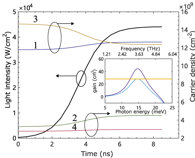
FIG. 5. In the four-well phonon–photon–phonon design shown in Fig. 2. Temporal evolution of the carrier density (right axis) and the light intensity (left axis) of the optical mode with the transition energy E_{32} = 14.3 \text{ meV} (3.46 THz). The inset is the unsaturated gain and the saturated gain spectrum. In this simulation T_e = T_l = 77 \text{ K} , cavity loss is set to be 28 \text{ cm}^{-1} , optical confinement factor \Gamma^{\text{opt}} = 1 , and interface roughness parameter are \Delta_{\text{IFR}} = 1.6 \text{ \AA} \Lambda_{\text{IFR}} = 100 \text{ \AA} .
