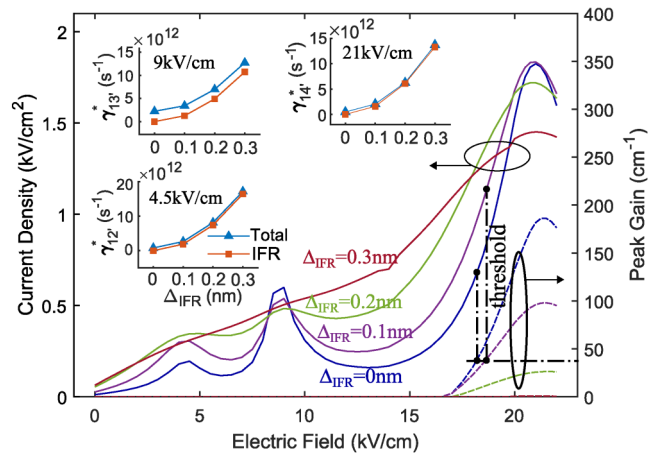
FIG. 9. I - V and peak optical gain vs the electric field of V843 for varying \Delta_{\text{IFR}} from 0 to 0.3 nm, \Delta_{\text{IFR}} = 10 nm. The three insets are the total and IFR pure dephasing rate of 1-2', 1-3', and 1-4' at their alignment electric field of 4.5, 9, and 21 kV/cm, respectively.
