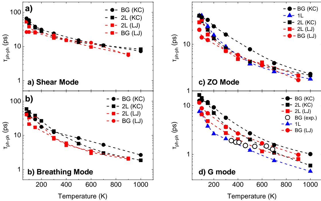
FIG. 7. The calculated temperature dependence \tau^{\text{ph-ph}}(T) of phonon lifetimes for the interlayer (a) Shear (b) Breathing (c) ZO and (d) G mode in 2L (square symbols) and graphite (round symbols), using KC (black full symbols) and LJ (red crossed symbols) as interlayer potentials. For the G-mode, the experimental data for graphite from Chatzakis et al [40] are also presented (hollow circles). Dashed lines connecting points are b-splines as visual guides.
