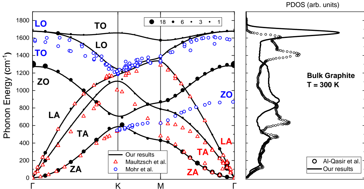
FIG. 1. (Left) The calculated phonon dispersion curves of Bulk Graphite (full symbols) at T = 300\text{ K} , together with data from IXS measurements (open symbols) [28, 64]. The magnitude of the kVACS symbols is a measure of the calculated lifetime. Straight lines connecting points are b-splines serving as visual guides. (Right) The calculated phonon DOS for Bulk Graphite at T = 300\text{ K} (straight lines), along with data from INS measurements [65] (open symbols). All PDOS are normalized to unit area.
