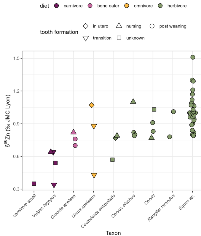
Extended Data Fig. 2 | Zinc stable isotope values across the Ranis food web. Zinc stable isotope ratios of a range of taxa show typical trophic relationships with low \delta^{66}\text{Zn} values for carnivores, high values for herbivores and intermediate omnivores and bone eating carnivores. Herbivores show a pattern with highest \delta^{66}\text{Zn} values in equids and lower values in typical browser to mixed feeding cervid taxa such as Cervus elaphus . This is potentially consistent with grazer-browser \delta^{66}\text{Zn} patterns observed in a European Pleistocene food web 38 and a modern
