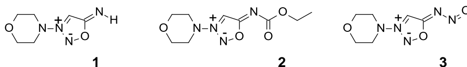
39 Figure 1. Molecular structures of SIN-1 ( 1 ), Mosildomine ( 2 ) and of 40 N -nitrosomorpholinosydnimine ( 3 ). 41 42
