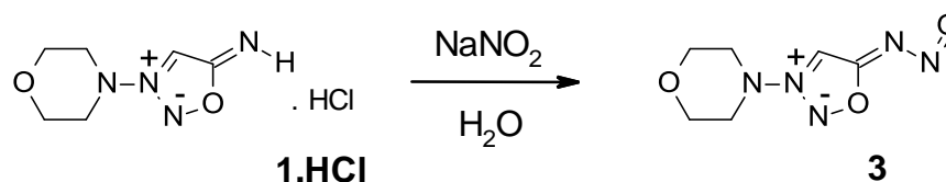
Scheme 1. Synthesis of N -nitrosomorpholinosydnonimine (3) § .
