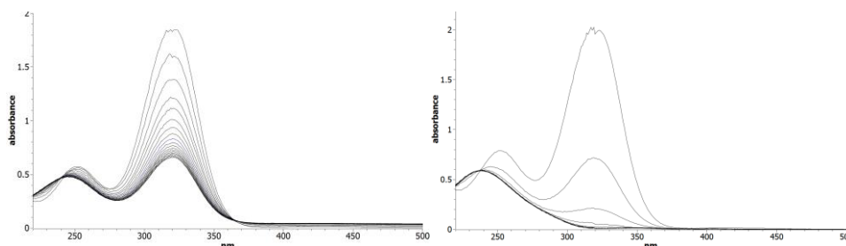
Figure 3. Repeated UV-visible spectral scans (30 min intervals) of decomposition of compound 3 (100 \mu\text{M} ) in aqueous solution of NaOH 2.5 mM (left) and 12.5 mM (right).
