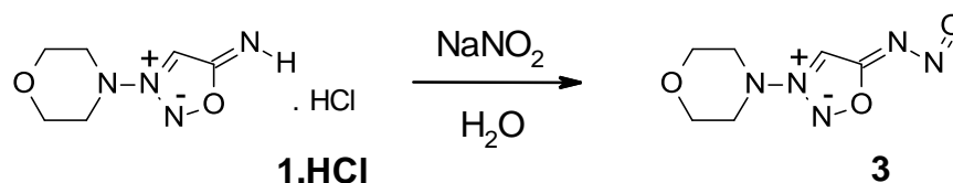
Scheme 1. Synthesis of N -nitrosomorpholinosydnonimine (3) § .
