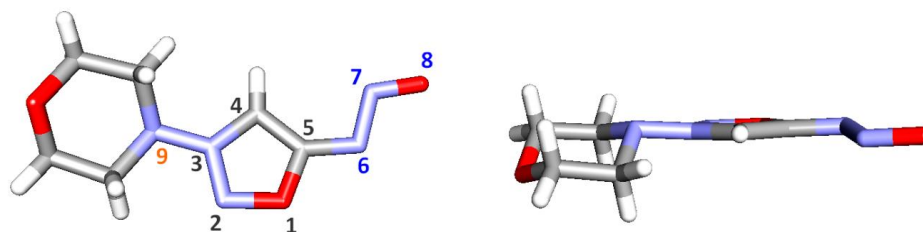
Figure 2. Two different views from X-ray structure of compound 3 and atom numbering (color code: C: gray, H: white, N: blue, O: red). See Table 1 (ESI) for crystal data (the cif file –CCDC 2381843– can be obtained free of charge from the Cambridge Crystallographic Data Center via https://www.ccdc.cam.ac.uk/ ).
