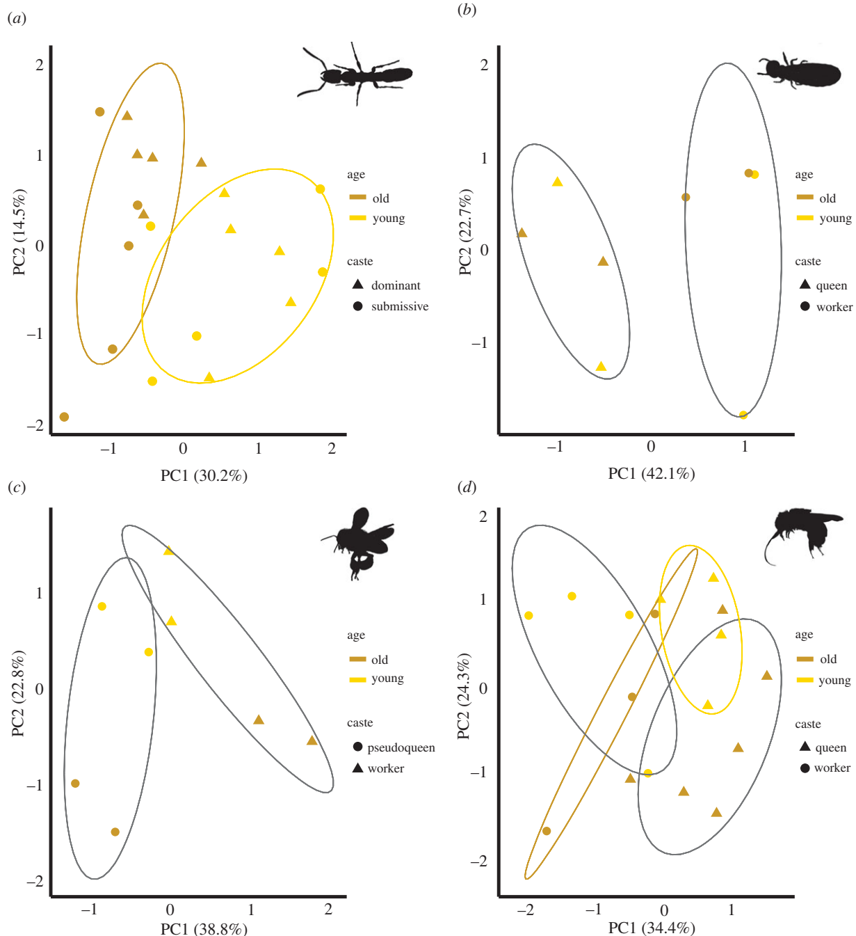
Figure 2. Results of principal component analyses (PCAs) based on the expression of the 20 candidate antioxidant genes common to the four species studied and presented by species: (a) the ant Platythreya punctata (abdomen), (b) the termite Cryptotermes secundus (whole body without guts), and the bees (c) Apis mellifera capensis (fat body of pseudoqueens and workers and (d) Euglossa viridissima (abdomen). Shown are the first (abscissa) and second (ordinate) principal components (PC) with variance explained by each PC. Each point represents the expression profile of one individual. Yellow shapes represent young and brown shapes old individuals, triangles represent reproductive individuals and circles, non-reproductive individuals. The ellipses displayed on the PCA plots highlight the main results of the PERMANOVA for each species (see main text), yellow/brown ellipses indicate an age effect, while black ellipses indicate a caste effect.
