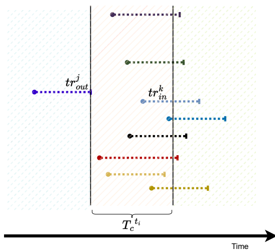
Figure 4: An illustration of conflict periods ( T_c^{\tau_i} )
