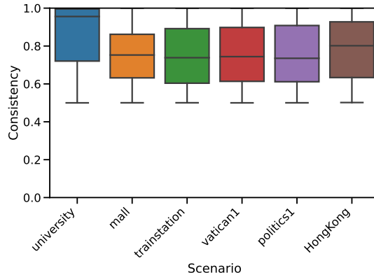
Figure 6: Consistency in time-based signatures
