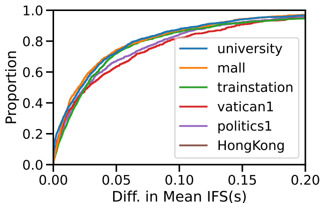
Figure 7: Difference in mean IFS.
