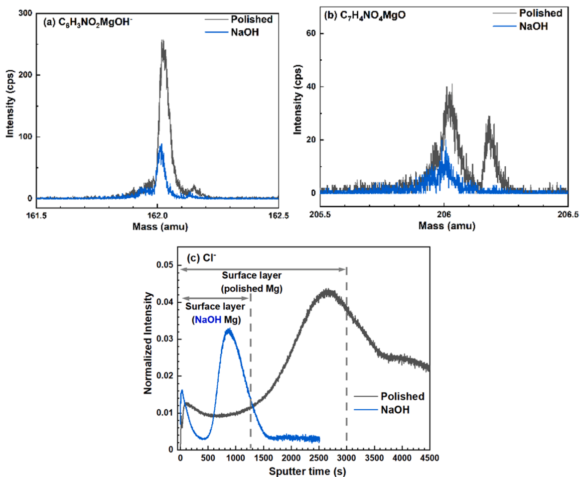
Fig. 8. Evolution of characteristic peaks in the mass spectra of 2,6-PDC at (a) 162.0041 amu ( C_6H_3NO_2MgOH^- ) and at (b) 205.9940 amu ( C_7H_4NO_4MgO ) and (c) profiles of Cl^- fragment obtained for polished (black) and NaOH-treated (blue) Mg samples. The signal is normalized by the sum of all signals.
