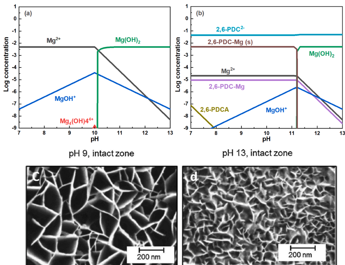
Fig. 15. Specie predominance diagram in NaCl aqueous electrolyte (a) without and (b) with 2,6-PDC 2- made using Hydra-Medusa. Input ions and their equilibrium concentrations: Mg 2+ (5 mM), Na + (58.5 mM) Cl - (8.5 mM), and 2,6-PDC 2- (50 mM). The stability constant of 2,6-PDC with Mg 2+ was found in [29] and added manually to Hydra-Medusa database, the solubility product of 2,6-PDC-Mg was replaced by that of MgCO 3 because there are no relevant parameters in the current database; typical ex-situ SEM micrograph of the Mg surface after 2 h of immersion in 0.1 M NaCl solution with different pH: 9 (c) and 13 (d). (c) and (d) were originally published by Maltseva et al. [57] and shown here for demonstration and reproduced with permission from Elsevier [57].
