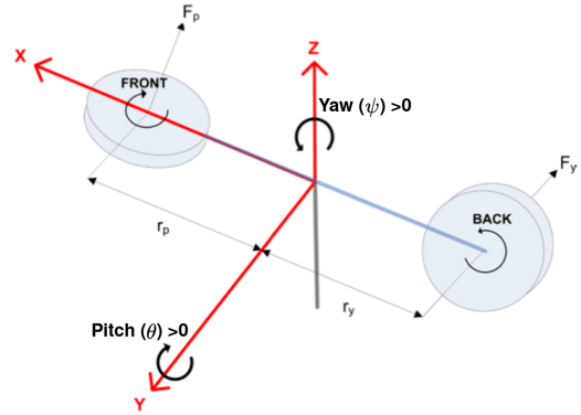
Figure 2: Free-body diagram of the Quanser Aero
