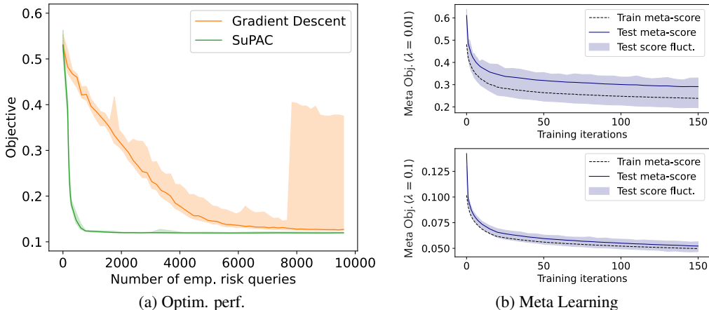
Figure 1: Experiments results. Figure 1a compares the optimisation performance of our algorithm SuPAC-CE with gradient descent approaches on an biochemical calibration task. Optimisation procedures were repeated 20 times; median performance and quantiles 0.2 and 0.8 are represented. Figure 1b investigates train and test performance of the meta-learning approach of Section 5. Mean test performance, as well as quantiles 0.2 and 0.8 for the sequence of built prior is assessed on 40 tasks and compared to the train performance. SuPAC-CE reduced the PAC-Bayes objective to 0.121 \pm 0.004 (avg. risk of posterior of 0.102 \pm 0.003 ).
