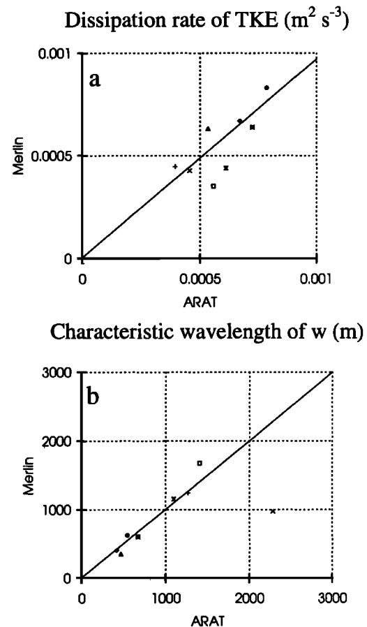
Figure 6. Comparison of the spectral characteristics. (a) Dissipation rate of turbulent kinetic energy (TKE) and (b) wavelength of the spectrum peak of the vertical velocity. See Figure 5 for the definition of the symbols.
