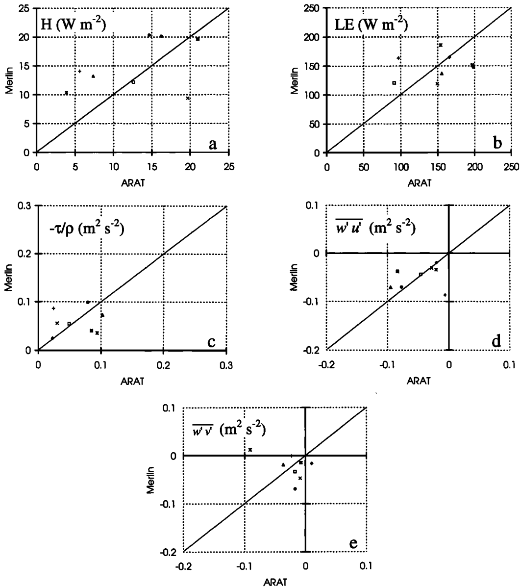
Figure 9. Comparison of (a) sensible heat flux, (b) latent heat flux, (c) total momentum flux (divided by the air density), (d) w'u' , and (e) w'v' covariances. Signals were high-pass filtered with a cutoff wavelength of 5 km. See Figure 5 for the definition of the symbols.
