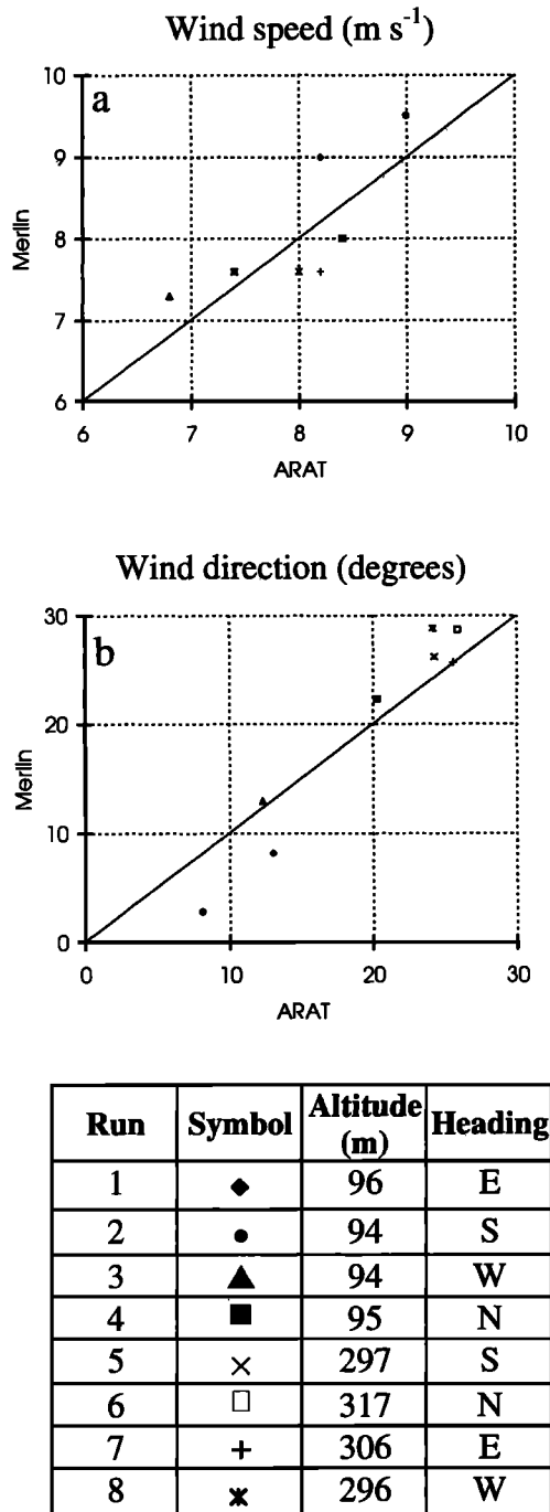
Figure 5. Comparison of (a) the mean wind speed and (b) direction computed on the eight straight and level runs. The correspondence between the symbols and the runs of the pattern are indicated.
