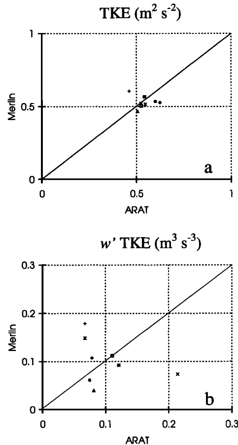
Figure 11. Comparison of (a) TKE (per unit mass) and (b) its vertical flux for high-pass filtered signals with a cutoff wavelength of 5 km. See Figure 5 for the definition of the symbols.
