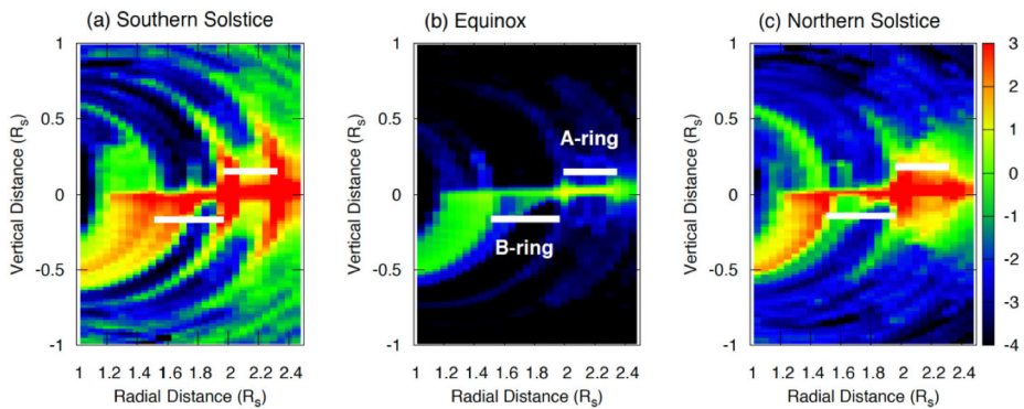
Fig. 19 O_2^+ ion density ( cm^{-3} ) in \log_{10} scale as indicated by the color bar at right for the three seasons and neutral O_2 source rates in Fig. 18: (a) Southern Solstice (SOI), (b) Equinox and (c) Northern Solstice (Grand Finale). (Tseng et al. 2010; Tseng and Ip 2011; Tseng et al. 2013a)
