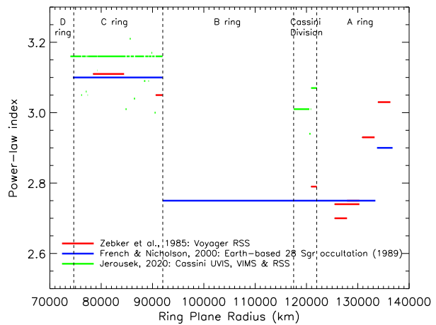
Fig. 3 Particle size distributions across Saturn's main rings: power-law indices inferred from Voyager RSS data (Zebker et al. 1985), 28 Sgr Earth-based occultation (French and Nicholson 2000), and Cassini UVIS, VIMS and RSS (Jerousek et al. 2020)
