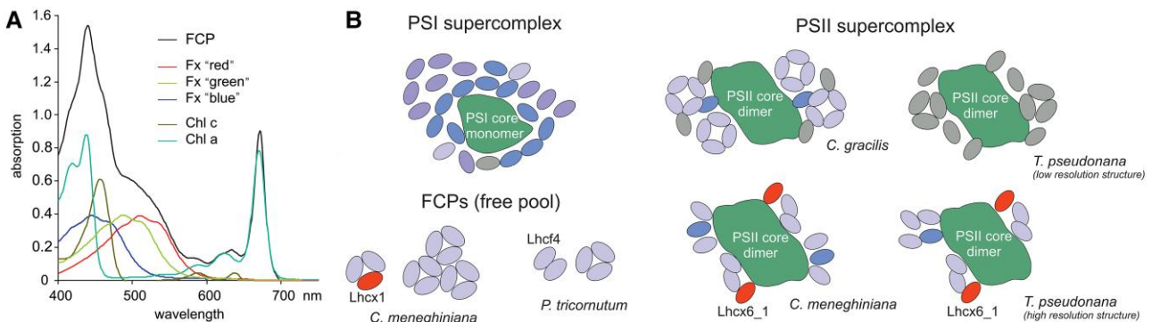
Figure 3. The FCP complex. A) Absorption spectrum of an FCP complex (black, FCPa from C. meneghiniana ) and its pigments. Fx molecules are bound at different sites, absorbing more to the red wavelength range (Fx “red”), intermediate (Fx “green”), or to the blue (Fx “blue”). B) Scheme of FCP arrangement in PSI, PSII, and the free FCP pool of different species. Lhc proteins are shown in red, other FCPs are colored according to their subfamily (light purple, Lhc4; blue, Lhc; purple, lhc; gray, unknown). For references, see text.
