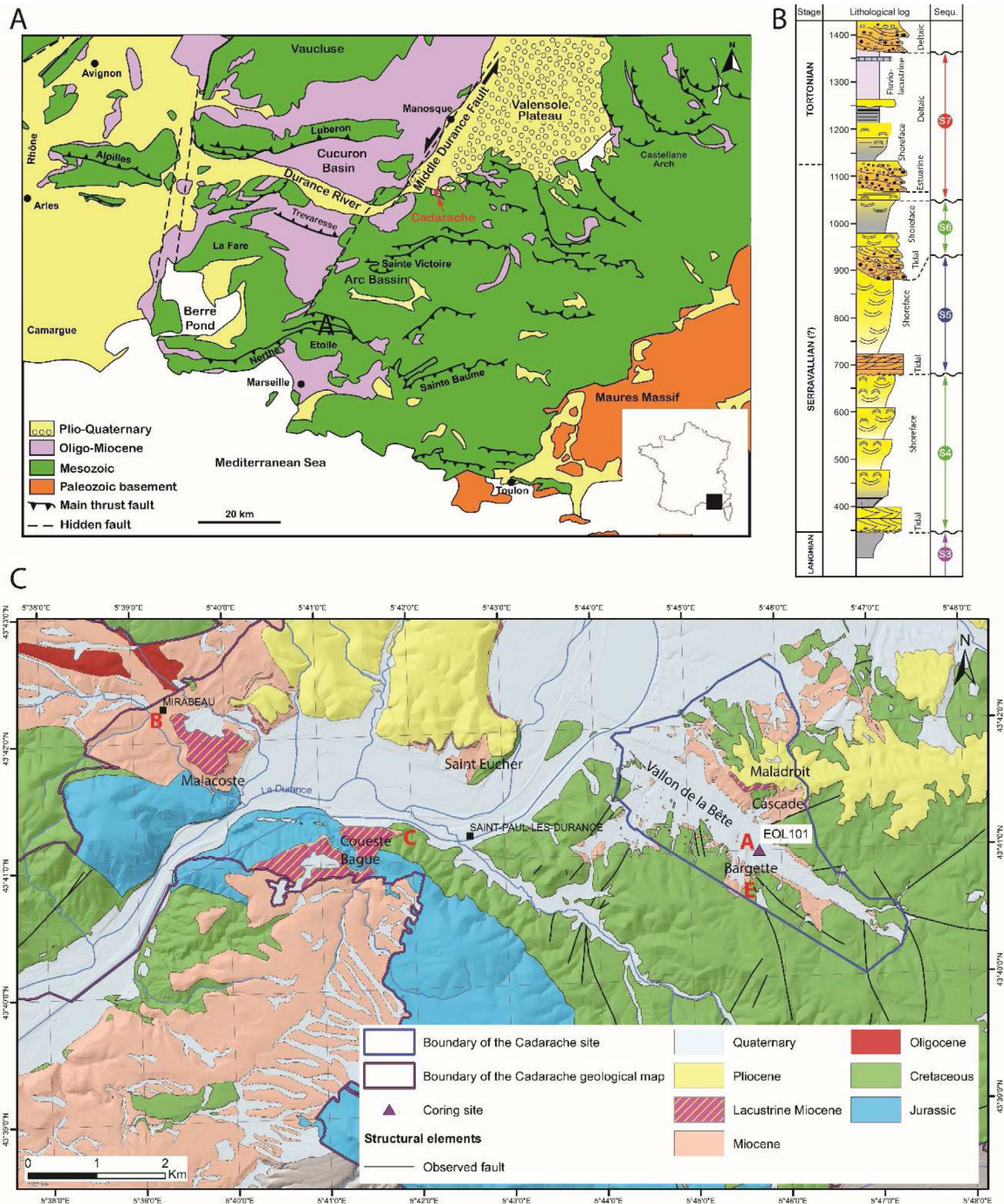
Fig. 1. A. Structural map of the Provence (modified after Demory et al., 2010); B. Synthetic log of the upper part of the Miocene in Provence (modified after Besson et al., 2005 and references therein). C. Geological map based on the geological map of Pertuis (Gouvernet et al., 1970) in its southwest and northwest parts and revised for the rest of the map (Guyonnet-Benaize, 2011 and references therein), with location of core EOL101 (A) and keys outcrops (B to E).
