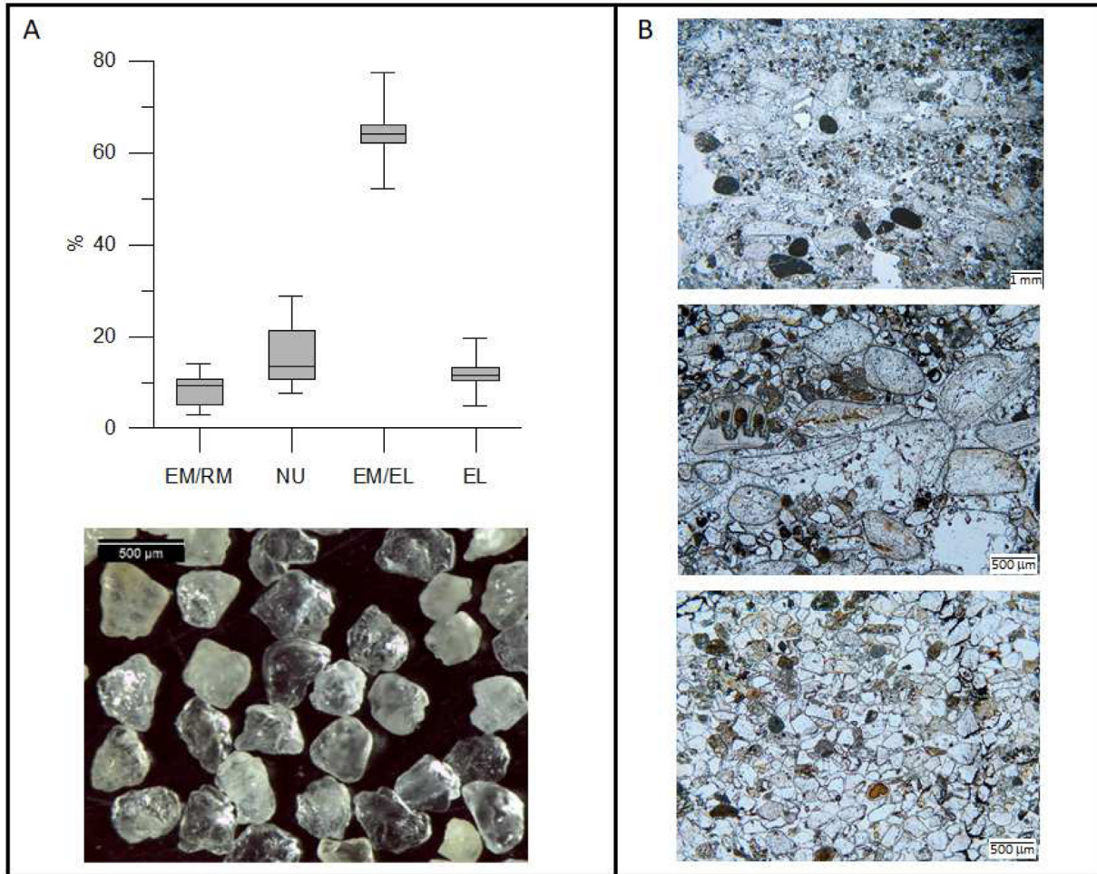
Fig. 4. A. Bar chart showing the proportion of the different grain surfaces after morphoscopic study led on 5 selected samples and a picture showing the most common quartz grain surfaces. B. Thin section pictures of samples collected from 2 carbonates-rich layers at 42 m-depth (picture on top and its close up in the middle) and at 4 m-depth (picture on the bottom).
