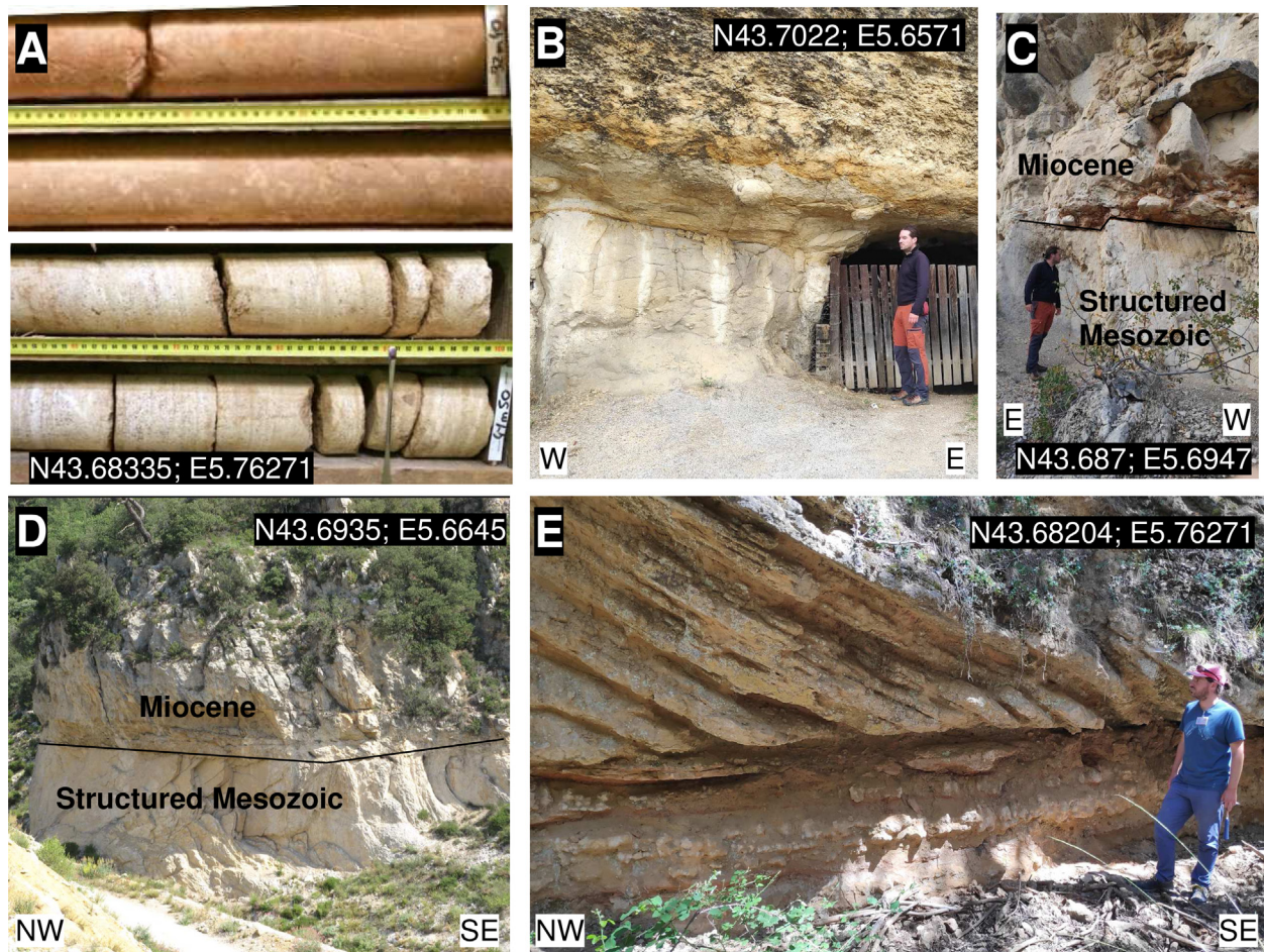
Fig. 2. Pictures of selected sections of core EOL 101 (A) and key outcrops: the Late Miocene marine sediments in Mirabeau area (B), transgressive surface on both side of the durance river (C and D) and a foresets sedimentary structure close to the core location (E).
