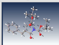
Ortep view of (2S,4R)-C4-benzyl-Theanine crystal
