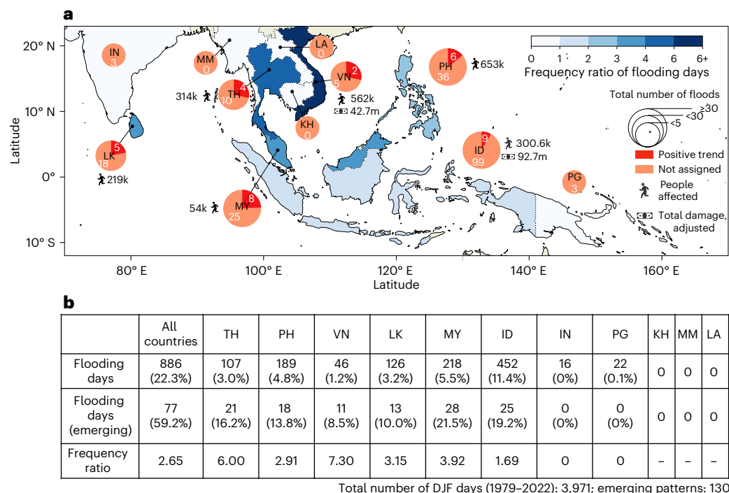
Fig. 3 | Impact of emerging weather patterns over the tropical Indo-Pacific region according to floods recorded in the EM-DAT database. a , The ratio of DJF flood days recorded under emerging weather patterns, compared with climatology. The sizes of the pie charts represent the total floods per country from 1979 to 2022, with red slices representing floods linked to emerging weather
