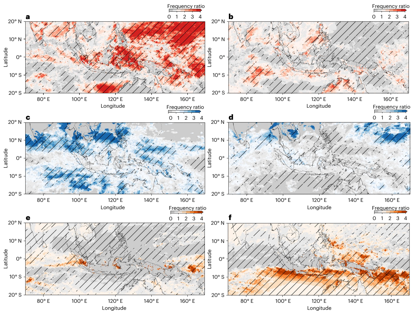
Fig. 2 | Weather extremes associated with emerging and disappearing weather patterns in DJF. a–f, Frequency ratio maps for heatwaves (a,b), extreme precipitation (c,d) and consecutive dry days (e,f) (Methods) as associated with emerging (a,c,e) and disappearing (b,d,f) weather patterns in DJF. Diagonal black
