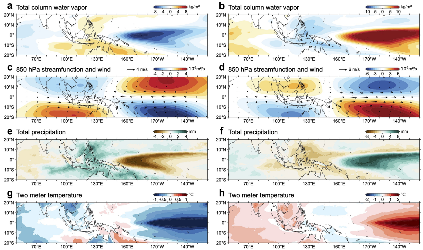
Extended Data Fig. 1 | Composite anomalies conditioned by the Niño3.4 index. The left column (a,c,e,g) depicts composite anomalies of La Niña, obtained using data with Niño3.4 index less than -1.5. The right column (b,d,f,h) depicts composite anomalies of El Niño, obtained using data with Niño3.4 index greater than 1.5.
