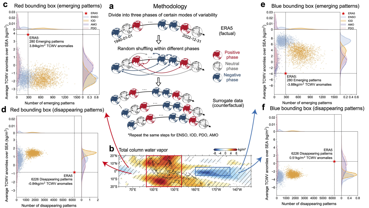
Extended Data Fig. 8 | Surrogate data study of the trend analysis. Plot (a) depicts a schematic representation of the framework for generating surrogate data through random shuffling of data applied within each phase (positive, neutral, negative) of each mode of variability considered in this study, that is, ENSO, IOD, AMO and PDO. The three colors of the Earth correspond to three different phases of a mode of variability, that is, red being positive, white neutral, and blue negative. The scatter plots (c,d,e,f) display results obtained from surrogate data for emerging patterns (c,e) and disappearing patterns (d,f), for
