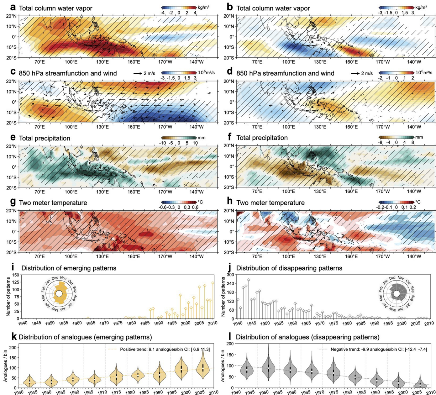
Extended Data Fig. 6 | Composite anomalies (a–h), for patterns with significant occurrence trends (i, j), and associated analogues (k, l), using TCWW as observable. As in Fig. 1, but for the ERA-20C reanalysis dataset. The ends of the boxes represent the 25th and 75th percentiles, with the whiskers
