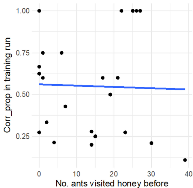
FIGURE A1 | Relation between the number of ants that entered the reward chamber before the tracked individual in their first training run ( n = 23 ) and correctness. The correctness is measured as the proportion of correct turns until the reward chamber is reached.
