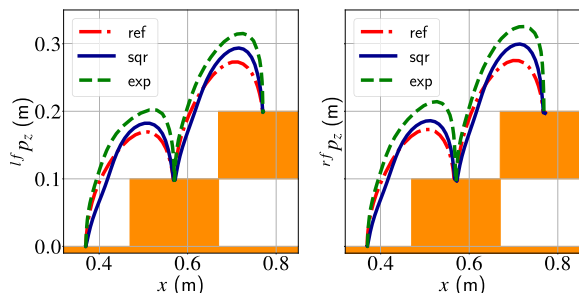
FIGURE 8. Feet trajectories, along the x and z directions, of ANYmal climbing two steps, obtained with the Ref method and the two fly-high costs.
